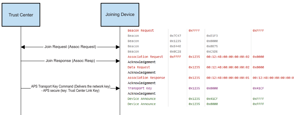
Figure 2. (a) Network Join Sequence When the Parent is the Trust Center (b) Ubiquita Log Snapshot Showing Over the Air Messages During Network Join Procedure
