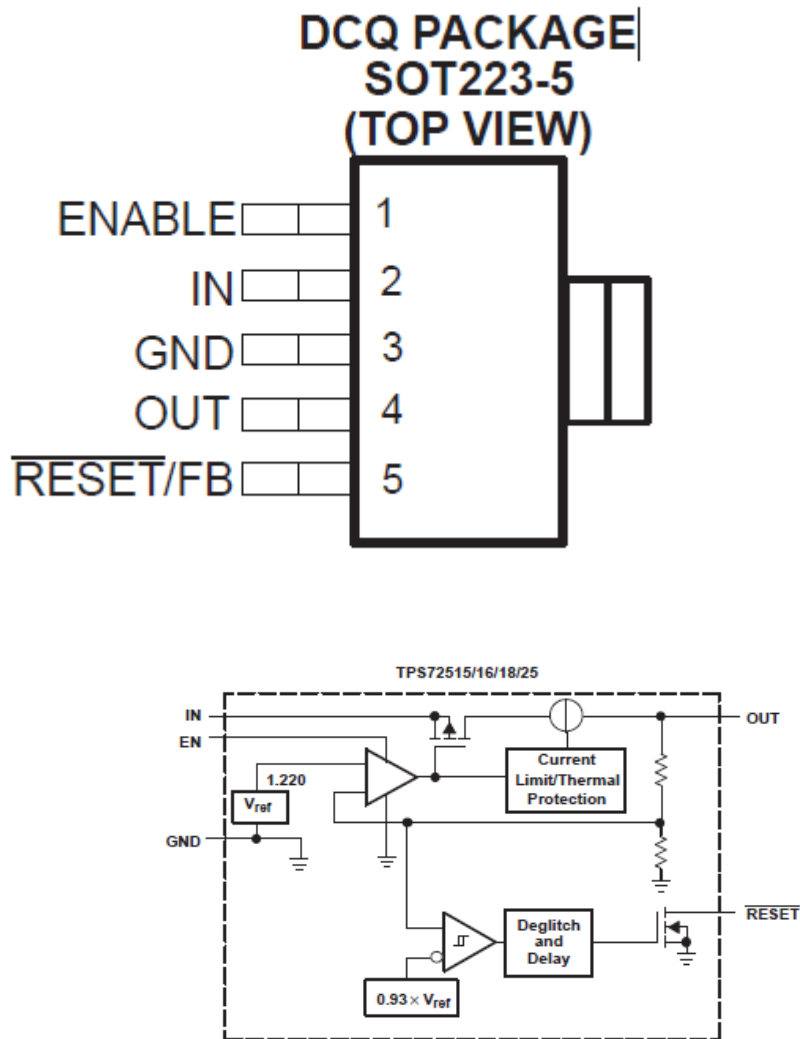
TERMINAL FUNCTIONS
