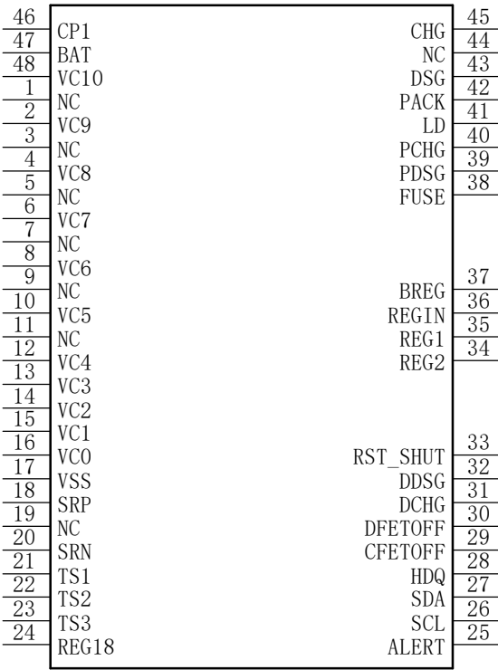
U5 BQ76942
