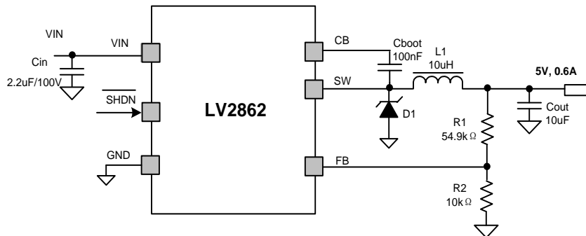
Application Circuit, 5V Output
