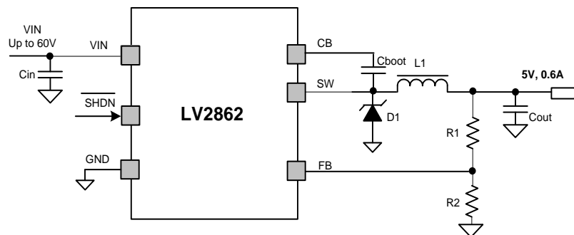
Typical application schematic
