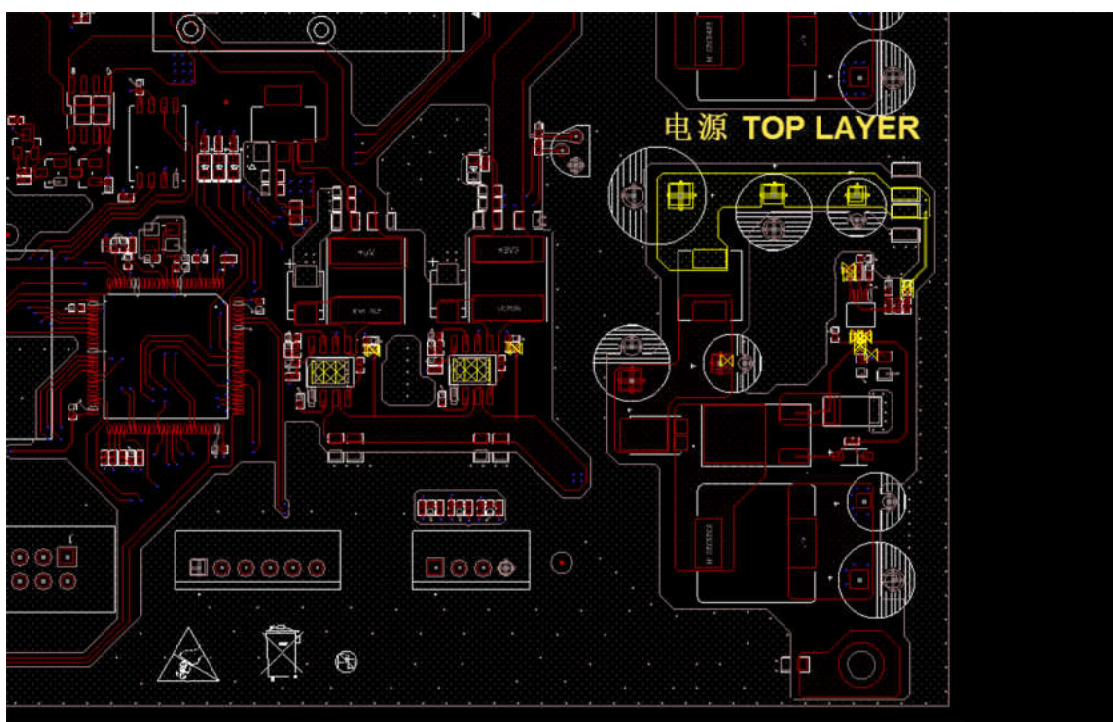
MP3910 LAYOUT
