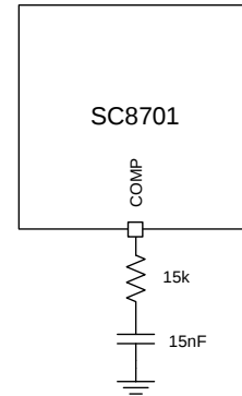
Figure 4 Feedback loop compensation setting
