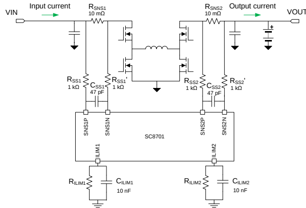
Figure 3 Input/output current monitoring circuit
