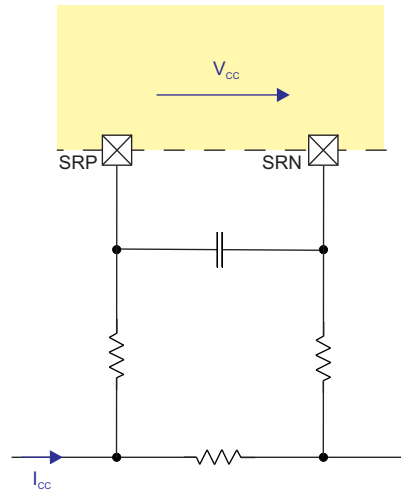
Figure 4. Current Calibration
