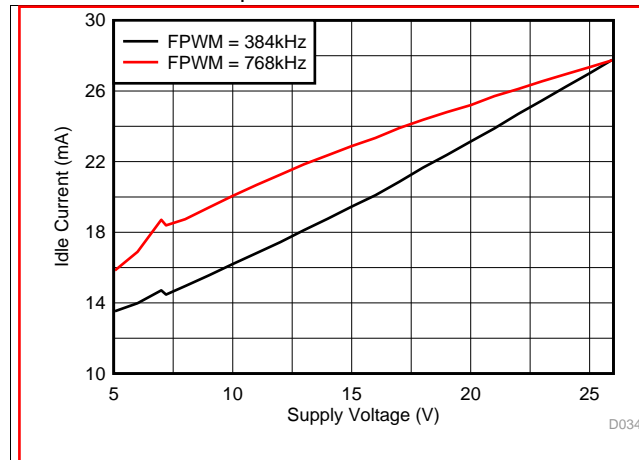
Figure 37. Supply Idle Current vs PVDD
