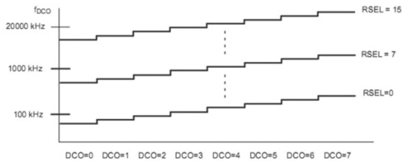
Figure 5-6. Typical DCOx Range and RSELx Steps
