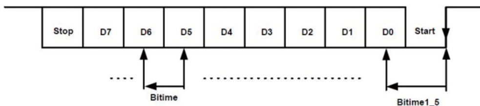
Figure 2. UART8N1 Character
