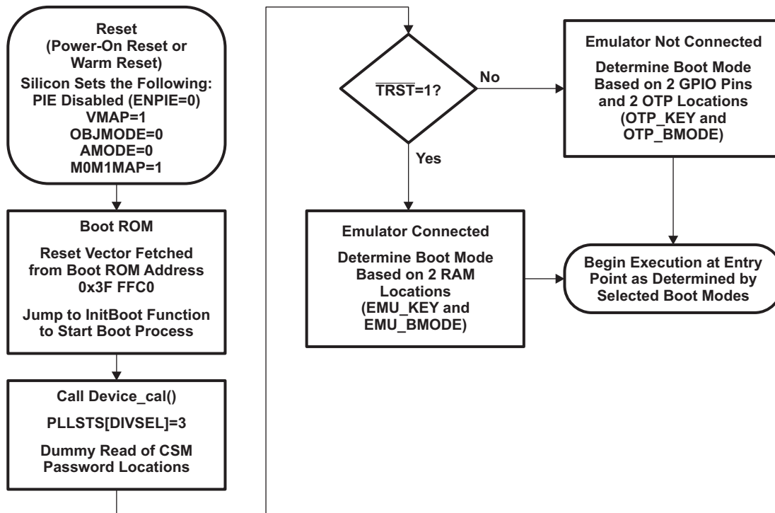
Figure 3. Bootloader Flow Diagram
