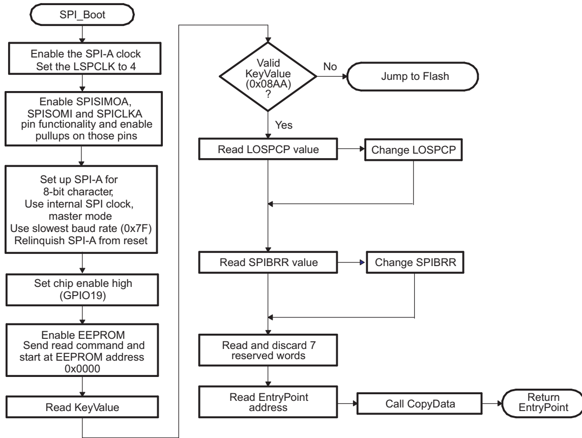
Figure 20. Data Transfer From EEPROM Flow
