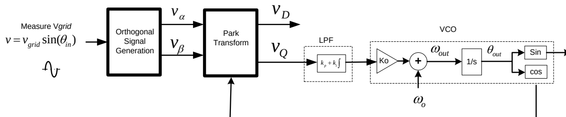
Figure 8 Phase Lock Loop Basic Structure
