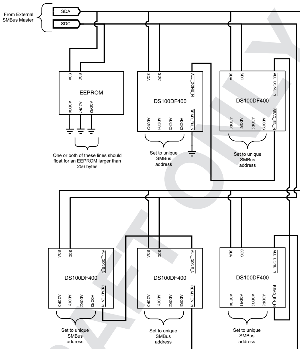
Figure 3. Connection Diagram for Multiple DS100DF400s in SMBus Master Mode
