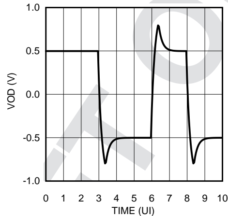
Figure 2. Idealized De-Emphasis Waveform
