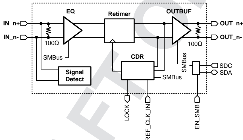
Figure 1. DS100DF400 Data Path Block Diagram — One of Four Channels
