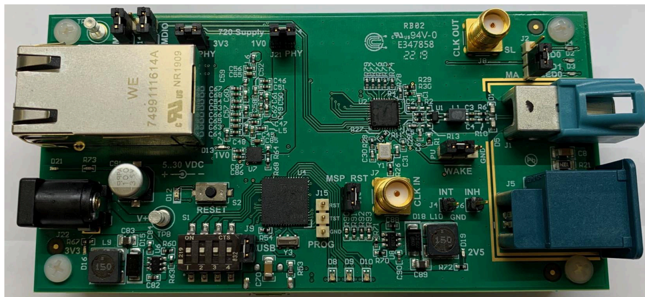
Figure 1-1. Ethernet Media Converter Board
