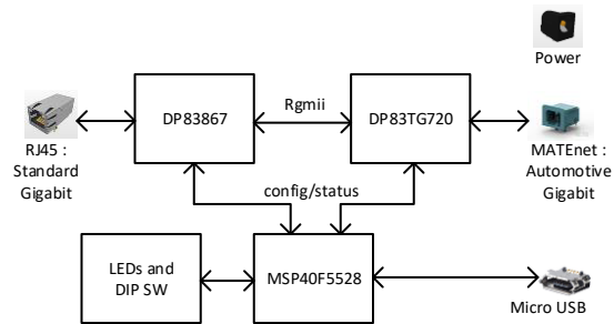
Figure 1-1. Block Diagram
