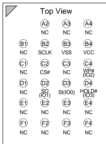
24-BALL TFBGA (6x4 ball array)
