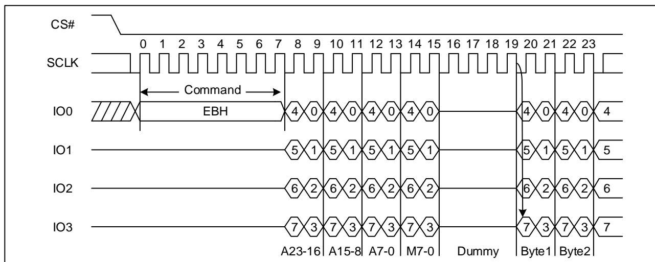
Figure 13. Quad I/O Fast Read Sequence Diagram ((M5-4) \neq (1, 0))
