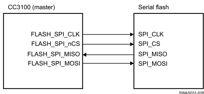
Figure 4-14. SPI Flash Interface
