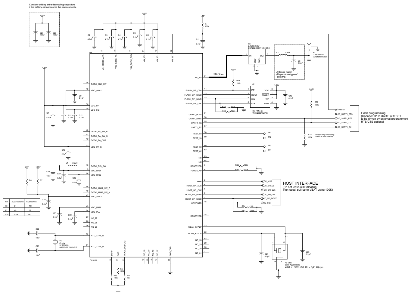
Figure 6-2. Schematics for CC3100 Preregulated 1.85-V Mode Application
