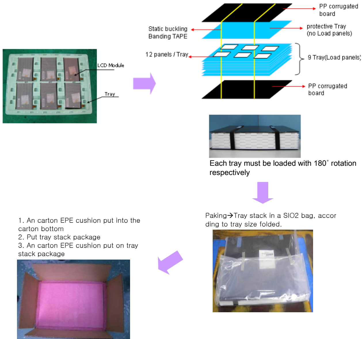
Figure9-1 Packing method
