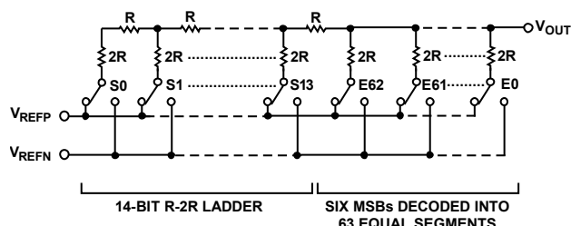
Figure 50. DAC Ladder Structure
