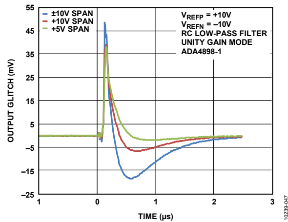
Figure 46. Midscale Peak-to-Peak Glitch for \pm 10 V
