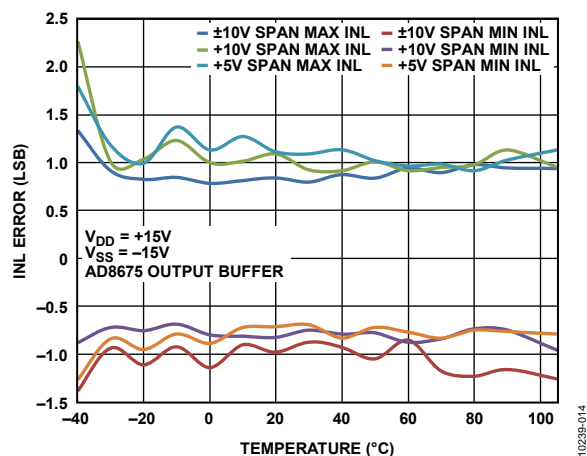
Figure 14. Integral Nonlinearity Error vs. Temperature
