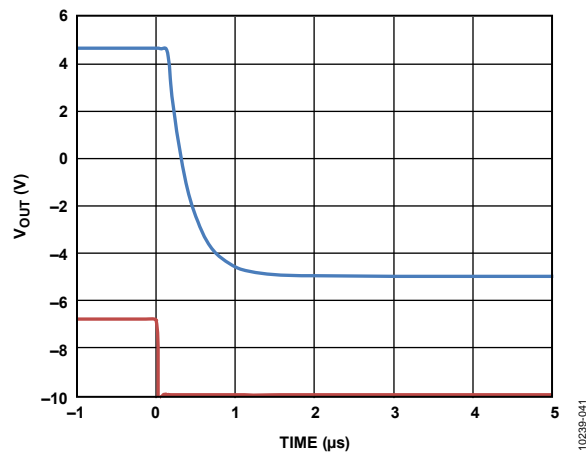
Figure 41. Falling Full-Scale Voltage Step
