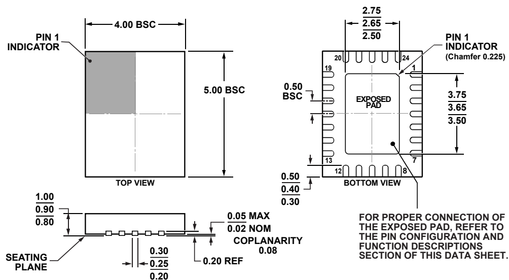
Figure 56. 24-Lead Lead Frame Chip Scale Package [LFCSP_VQ] 4 mm x 5 mm Body, Very Thin Quad (CP-24-5) Dimensions shown in millimeters
