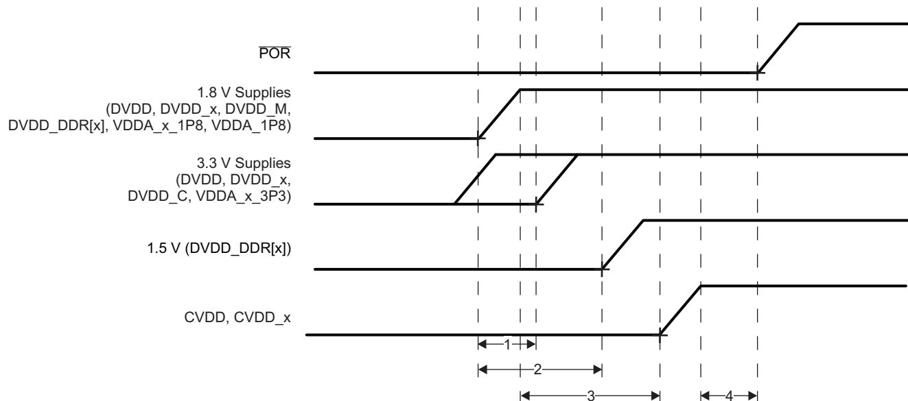
Figure 7-1. Power-Up Sequence
