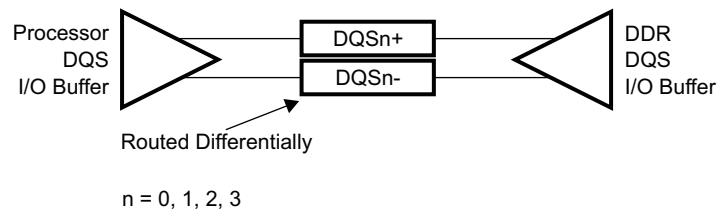
Figure 8-76. DQS Topology
