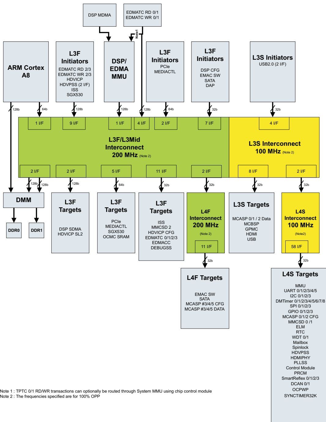
Figure 5-1. System Interconnect
