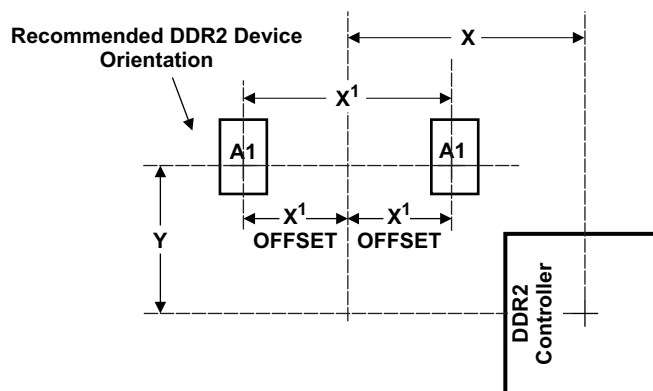
Figure 8-50. DM814x Device and DDR2 Device Placement
