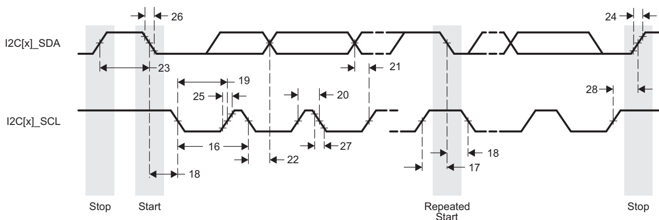
Figure 8-44. I2C Transmit Timing
