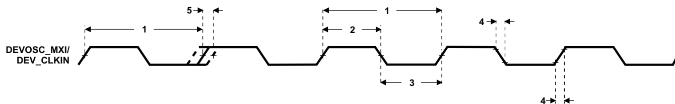
Figure 7-12. DEV_MXI/DEV_CLKIN Timing
