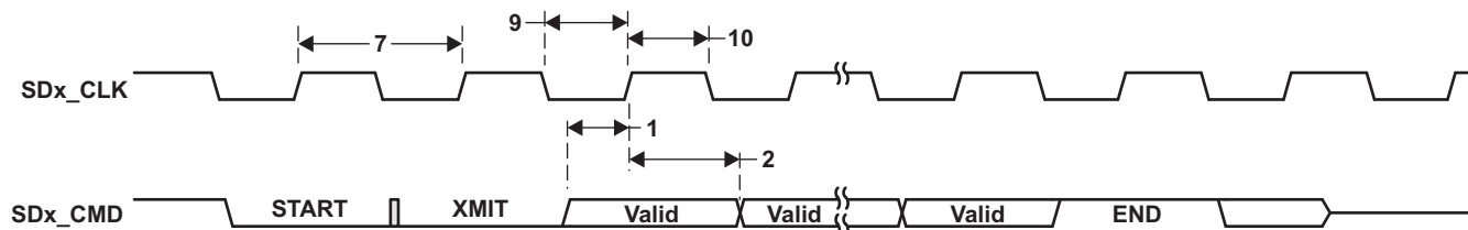
Figure 8-88. MMC/SD/SDIO Card Response Timing
