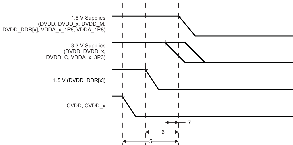
Figure 7-3. Power-Down Sequence
