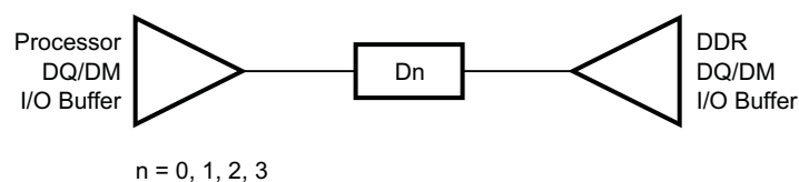
Figure 8-77. DQ/DM Topology
