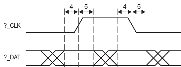
Figure 7-45 HyperLink Station Management Transmit Timing
