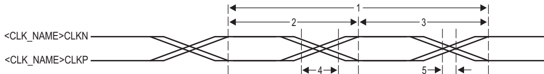
Figure 7-24 PLL Transition Time
