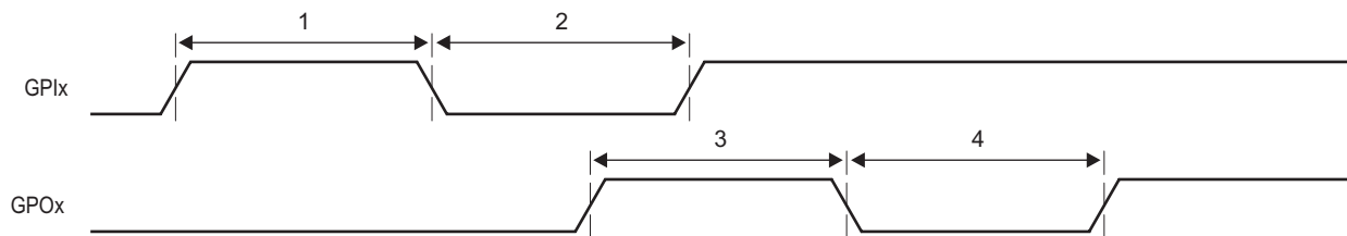
Figure 7-57 GPIO Timing
