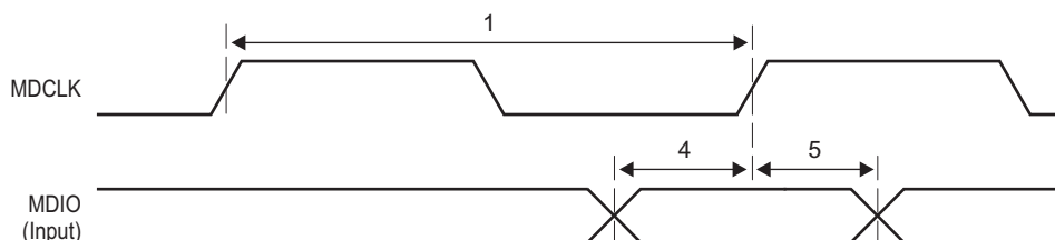
Figure 7-54 MDIO Input Timing
