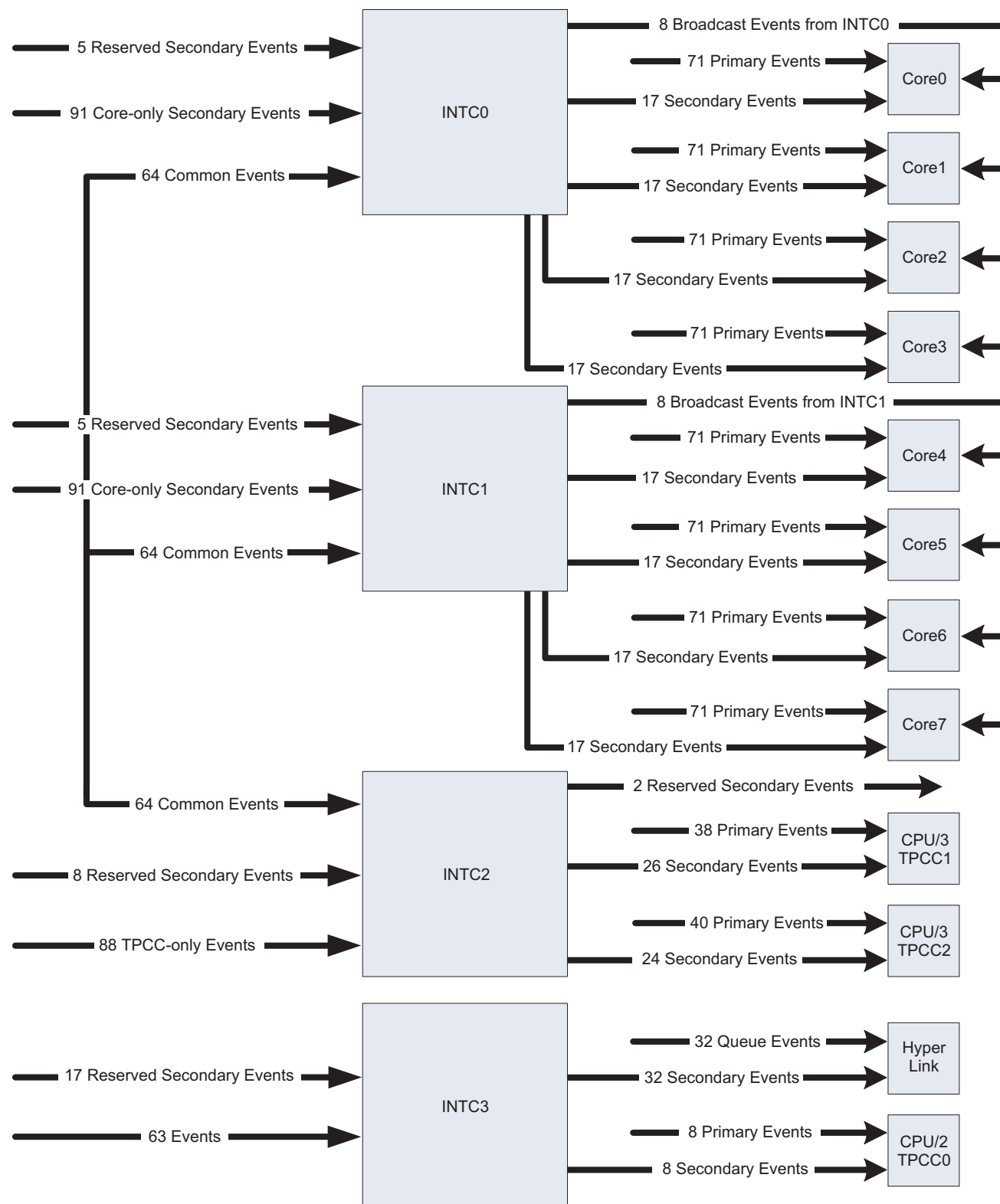
Figure 7-33 TMS320C6678 Interrupt Topology
