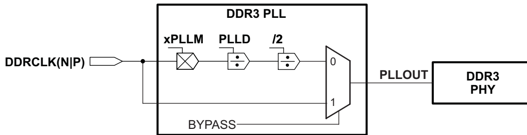
Figure 7-25 DDR3 PLL Block Diagram
