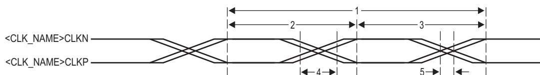
Figure 7-32 PASS PLL Timing
