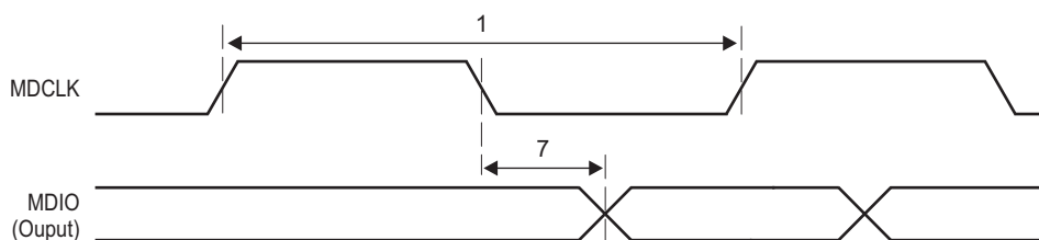
Figure 7-55 MDIO Output Timing
