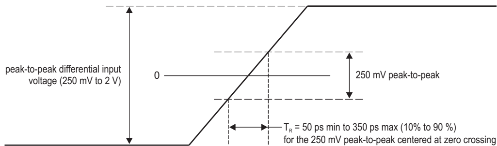
Figure 7-24 PLL Transition Time
