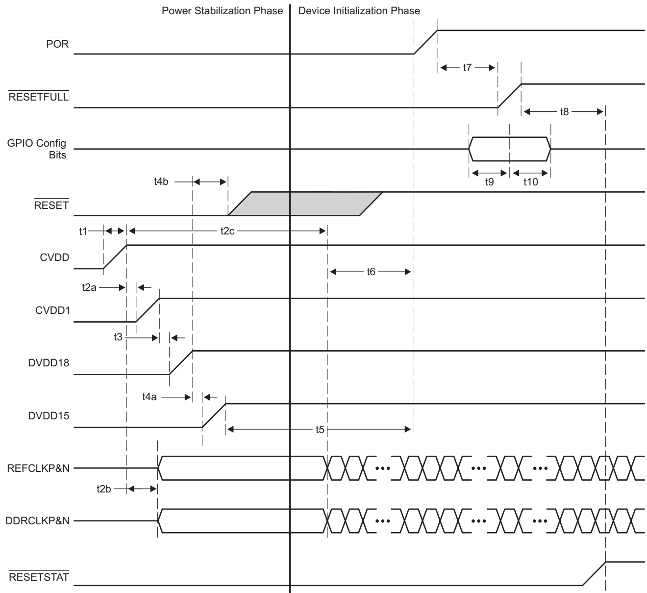
Figure 7-5 Core Before IO Power Sequencing
