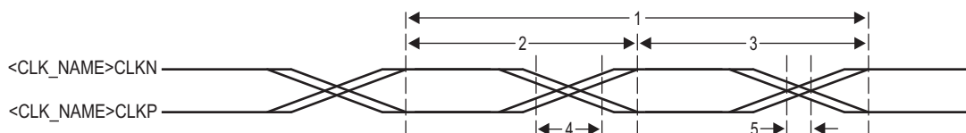
Figure 7-28 DDR3 PLL DDRCLK Timing
