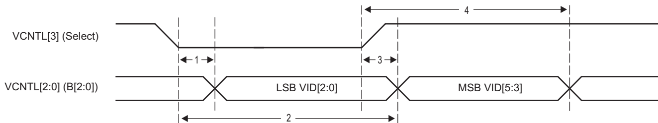
Figure 7-7 SmartReflex 4-Pin VID Interface Timing
