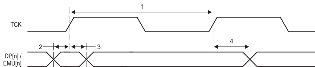
Figure 7-60 HS-RTDX Timing
