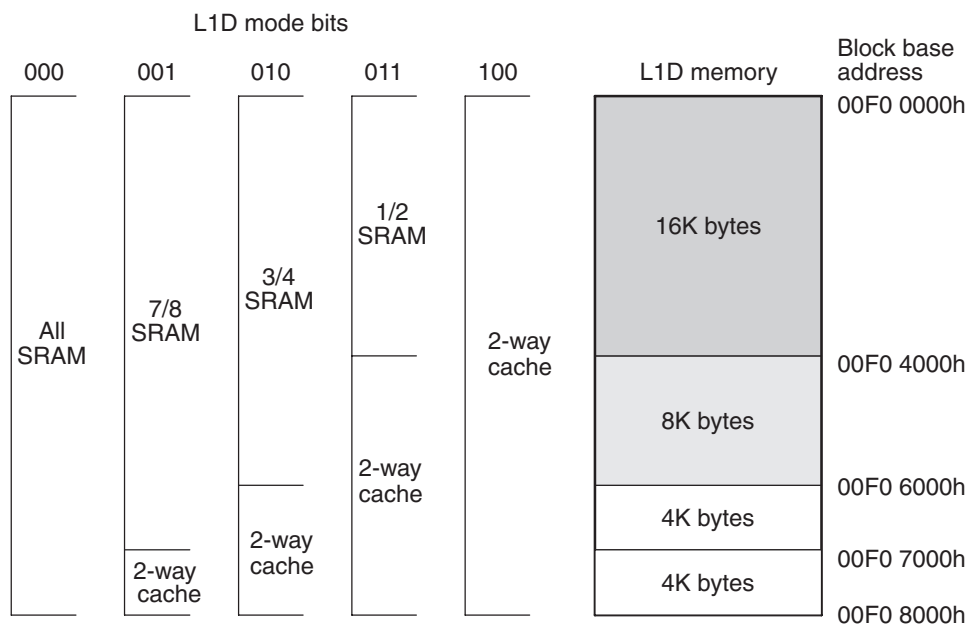
Figure 5-3 TMS320C6678 L1D Memory Configurations
