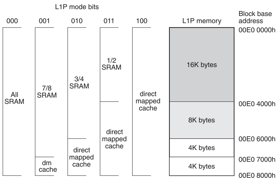
Figure 5-2 TMS320C6678 L1P Memory Configurations
