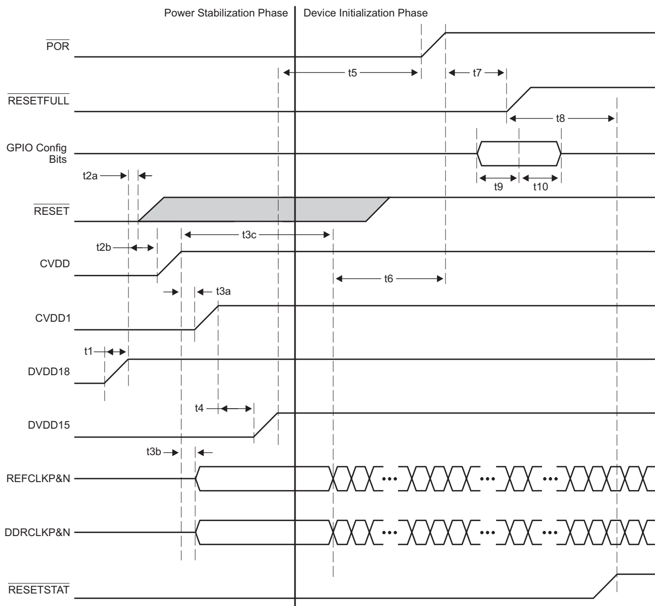
Figure 7-6 IO Before Core Power Sequencing
