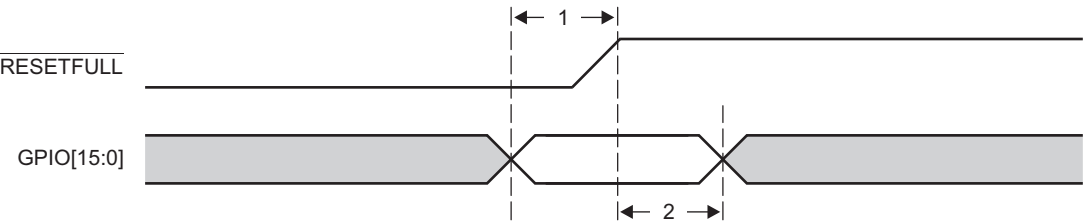
Figure 7-10 Boot Configuration Timing
