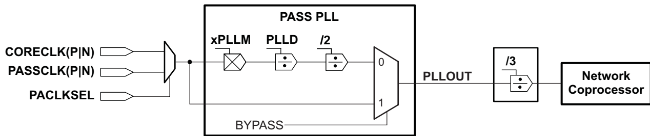
Figure 7-29 PASS PLL Block Diagram
