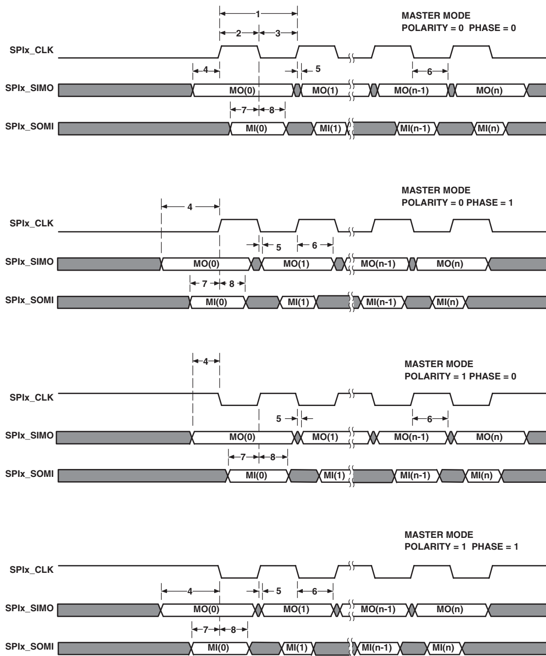
Figure 7-42 SPI Master Mode Timing Diagrams — Base Timings for 3 Pin Mode
