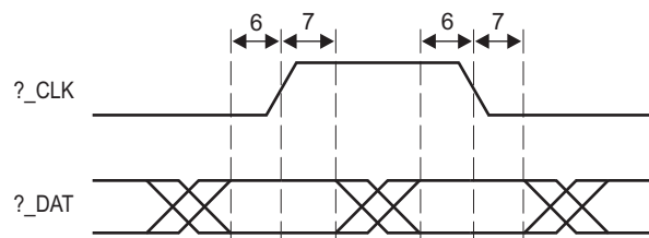
Figure 7-46 HyperLink Station Management Receive Timing
