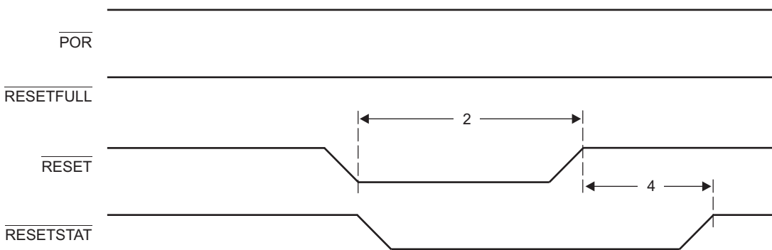
Figure 7-9 Soft/Hard-Reset Timing
