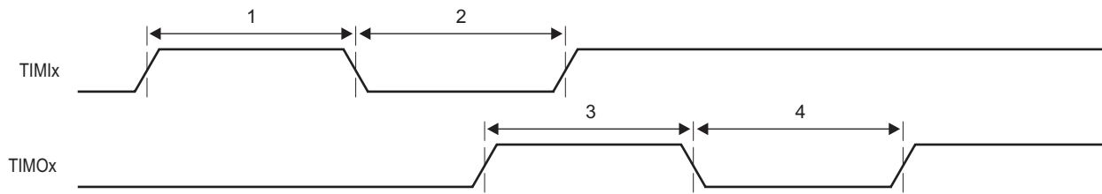
Figure 7-56 Timer Timing
