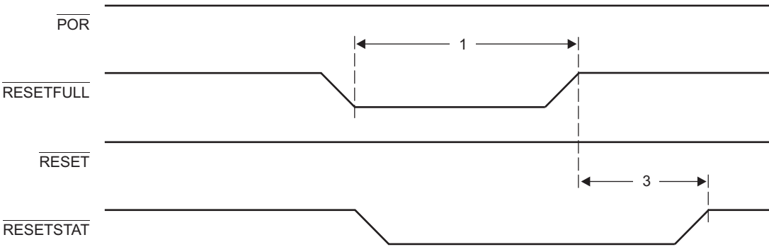
Figure 7-9 Soft/Hard-Reset Timing
