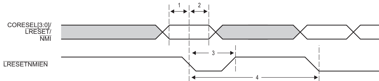
Figure 7-34 NMI and Local Reset Timing
