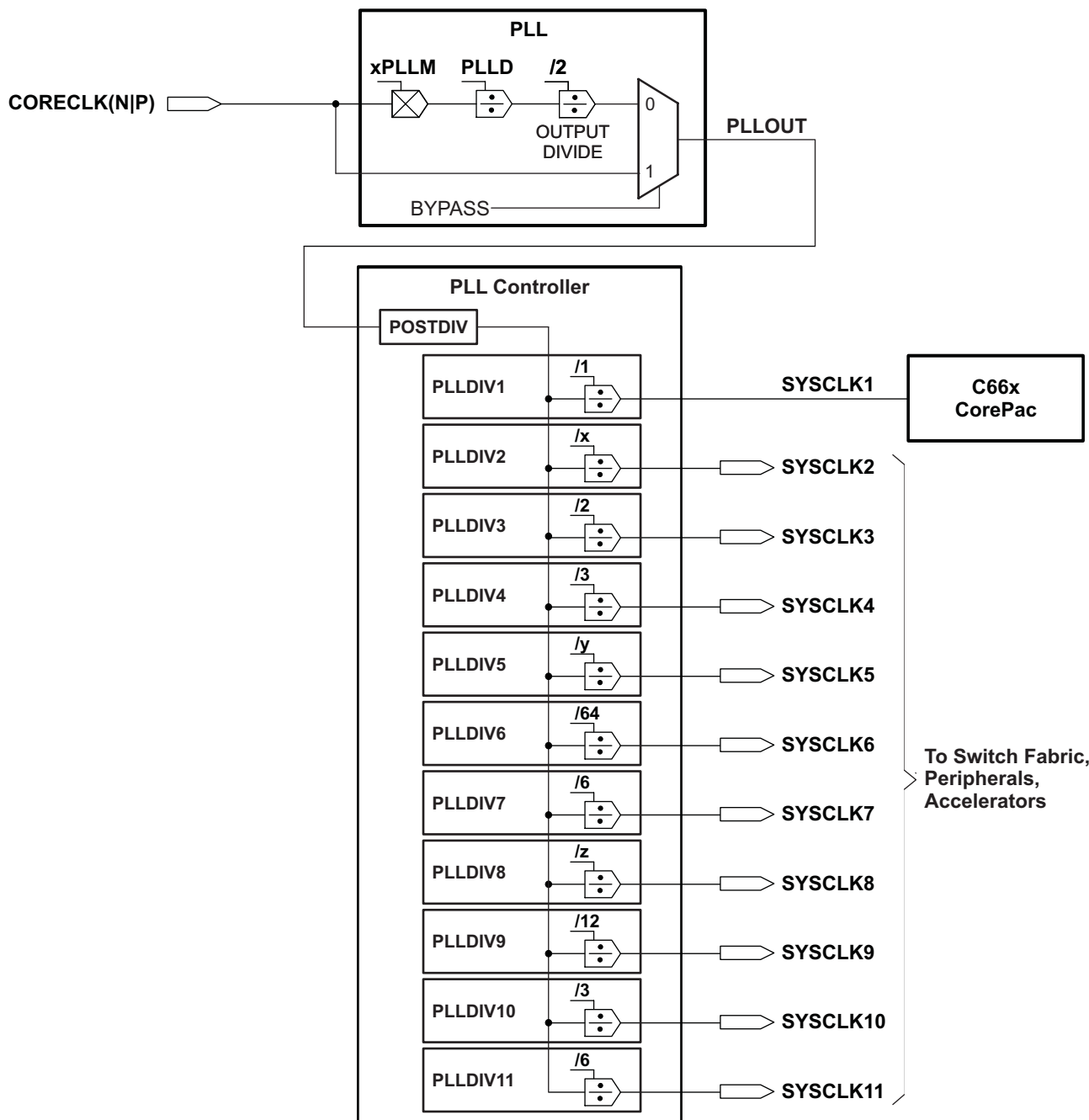
Figure 7-11 Main PLL and PLL Controller
