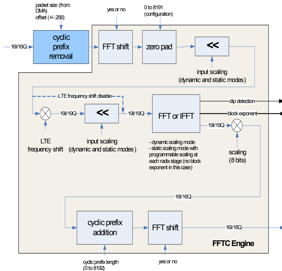
Figure 2-1 FFT Engine
