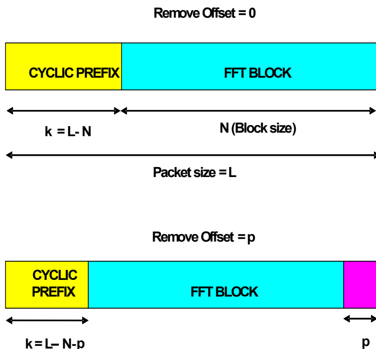
Figure 2-7 Cyclic Prefix Removal
