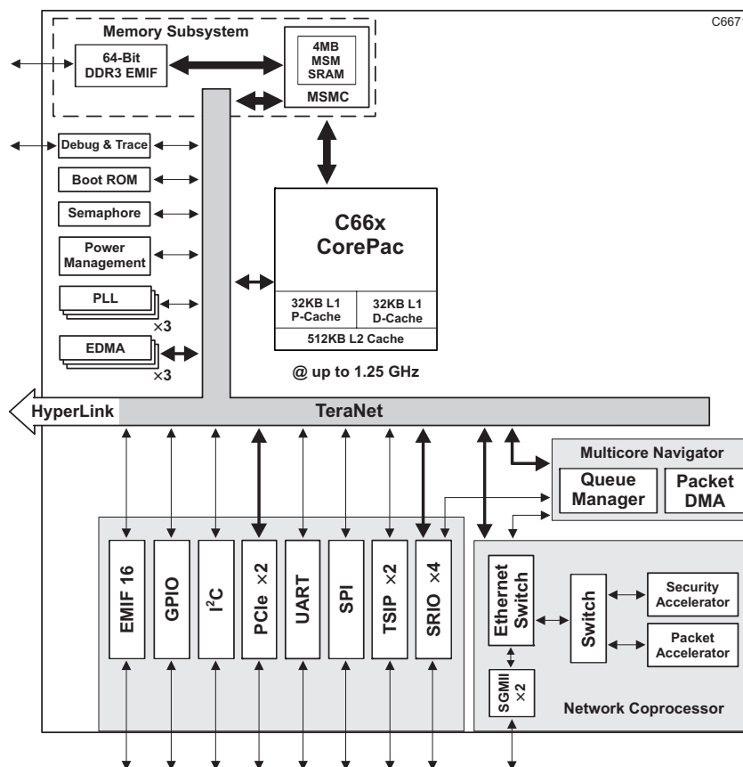
Figure 1 High-Level Block Diagram of TI's TMS320C6671 DSP
