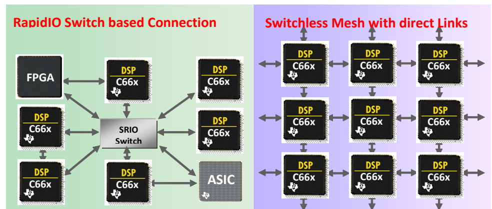
Figure 5 On-board Connectivity using Serial RapidIO
