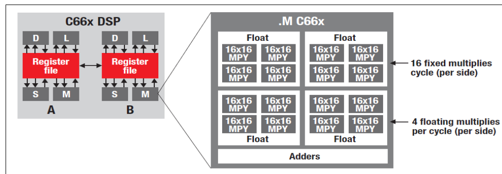
Figure 2 High-level View of the Execution Unit Within TI's C66x DSP Core with Respect to Multiply Operations
