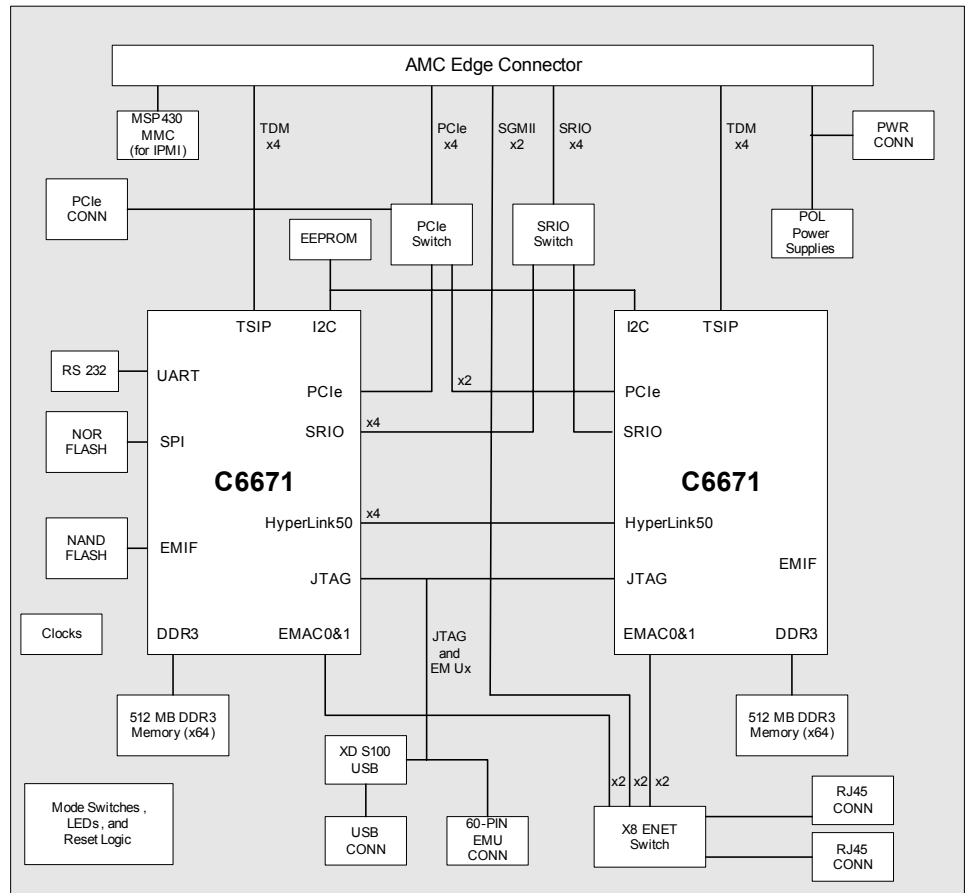
Figure 7 High-level View of TI's Dual C6671 DSP Hardware Design Solving Problems
