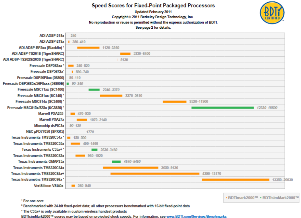
Figure 4 Fixed-point Speed Scores for the BDTI DSP Kernel Benchmarks
