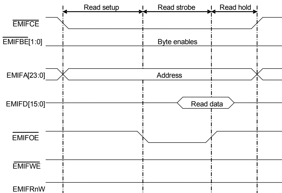
Figure 2-4 Asynchronous Read Timing Diagram
