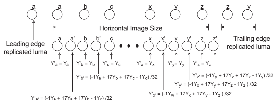
Figure 4-23. Luma Edge Replication
