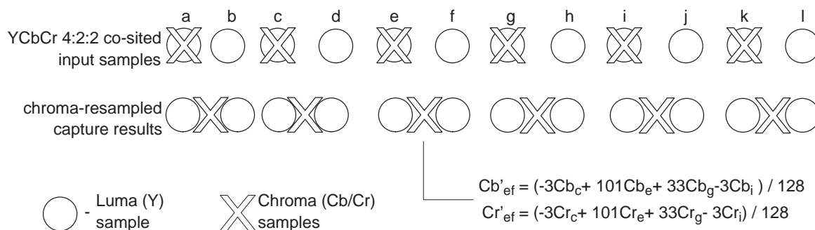
Figure 3-12. Chrominance Re-sampling
