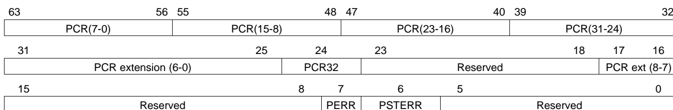
Figure 3-27. TSI Timestamp Format (Big Endian)
