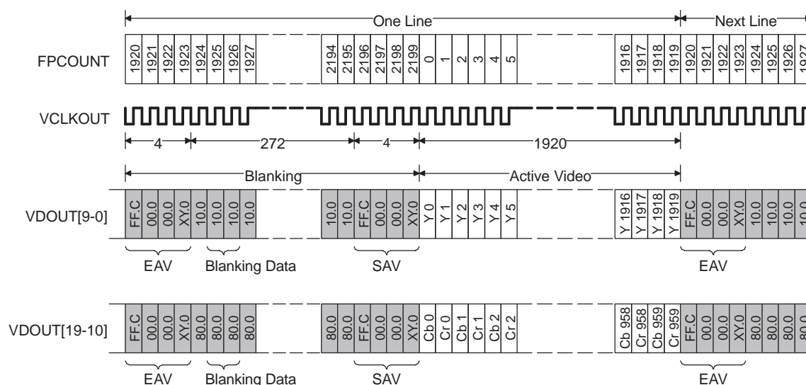
Figure 4-15. Y/C Horizontal Blanking Timing (BT.1120 60I)
