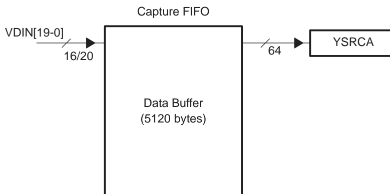
Figure 1-5. 16/20-Bit Raw Video Capture FIFO Configuration
