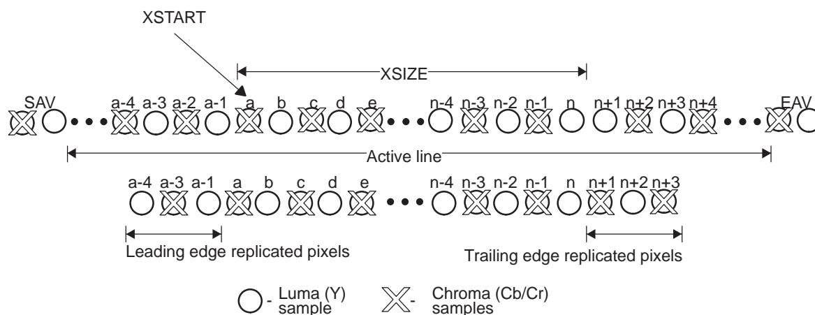
Figure 3-16. Capture Window Not Requiring Edge Pixel Replication
