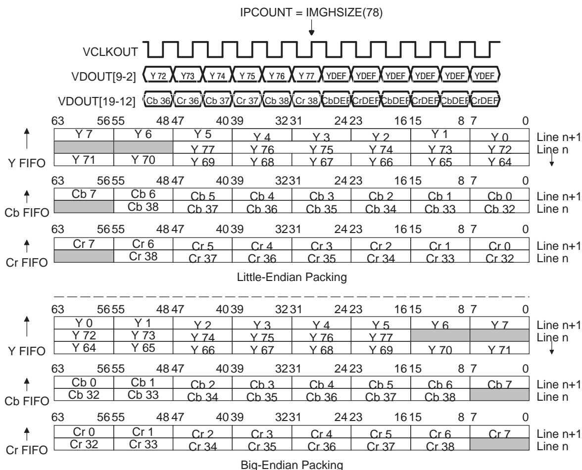
Figure 3-28. Capture Line Boundary Example
