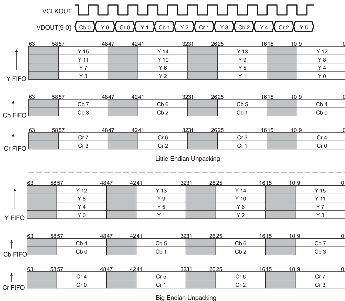
Figure 4-13. 10-Bit BT.656 FIFO Unpacking
