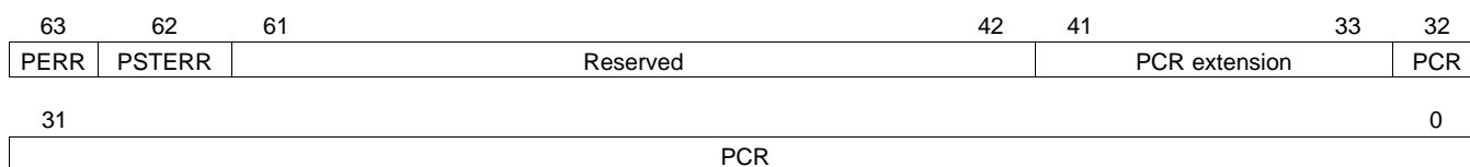
Figure 3-26. TSI Timestamp Format (Little Endian)
