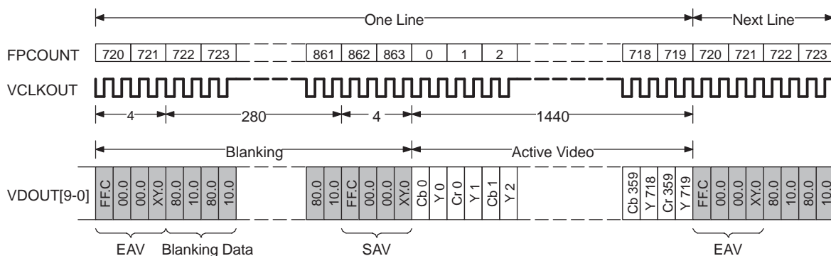
Figure 4-10. 625/50 BT.656 Horizontal Blanking Timing
