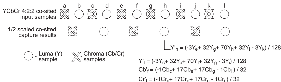
Figure 3-13. ½ Scaled Co-Sited Filtering
