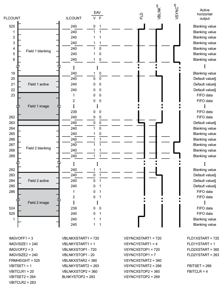
Figure 4-34. BT.656 Interlaced Display Vertical Timing Example
