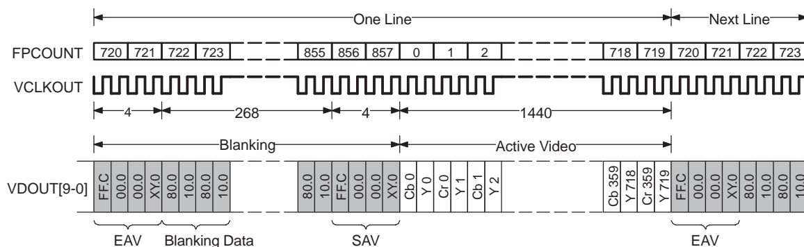
Figure 4-9. 525/60 BT.656 Horizontal Blanking Timing
