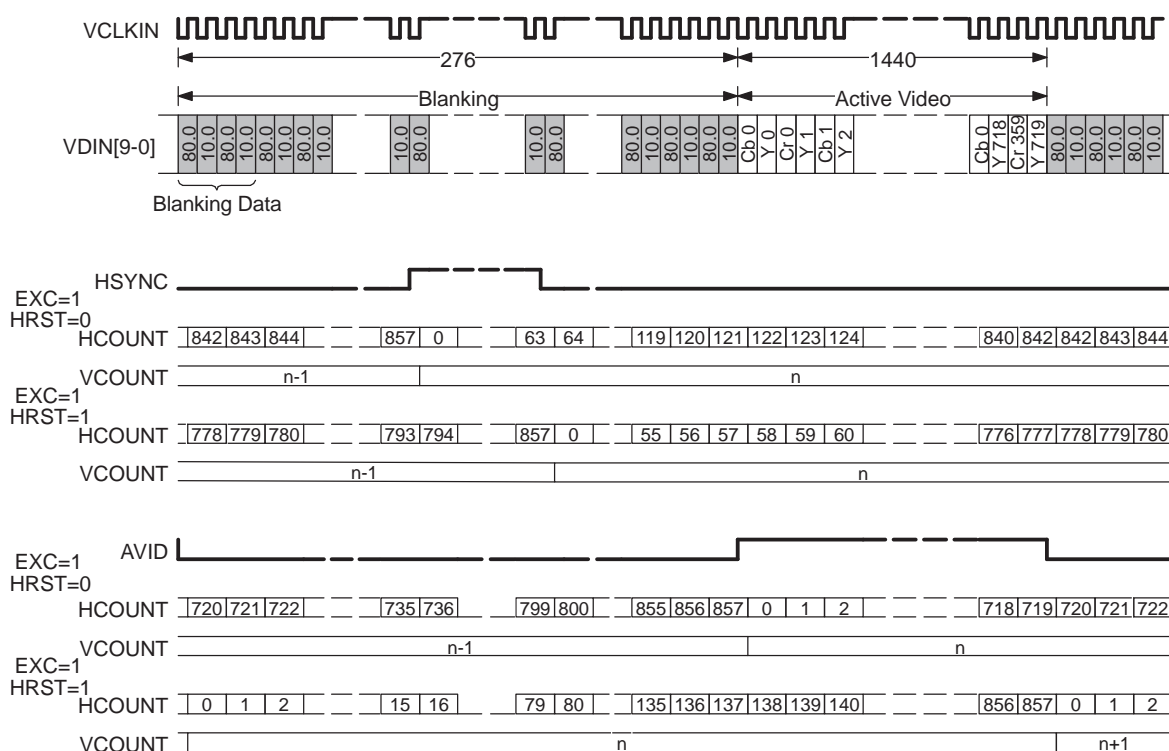
Figure 3-10. HCOUNT Operation Example (EXC = 1)
