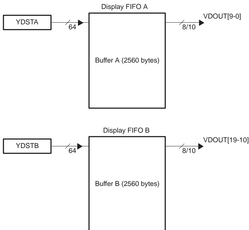
Figure 1-8. 8/10 Bit Locked Raw Video Display FIFO Configuration
