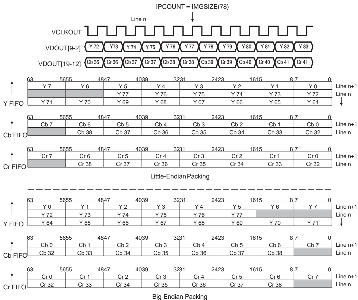
Figure 4-32. Display Line Boundary Example
