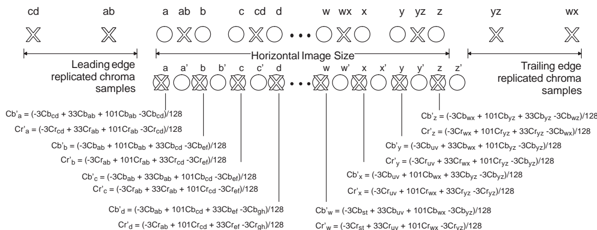
Figure 4-24. Interspersed Chroma Edge Replication
