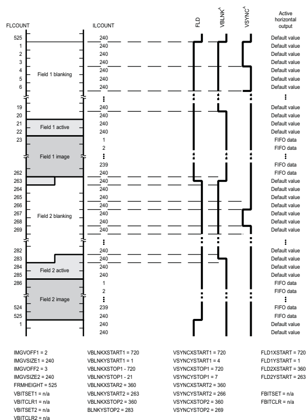
Figure 4-36. Raw Interlaced Display Vertical Timing Example
