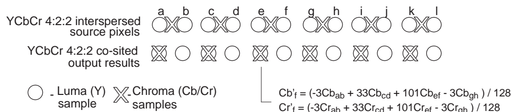
Figure 4-19. Chrominance Re-sampling
