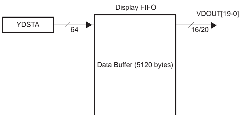
Figure 1-9. 16/20-Bit Raw Video Display FIFO Configuration
