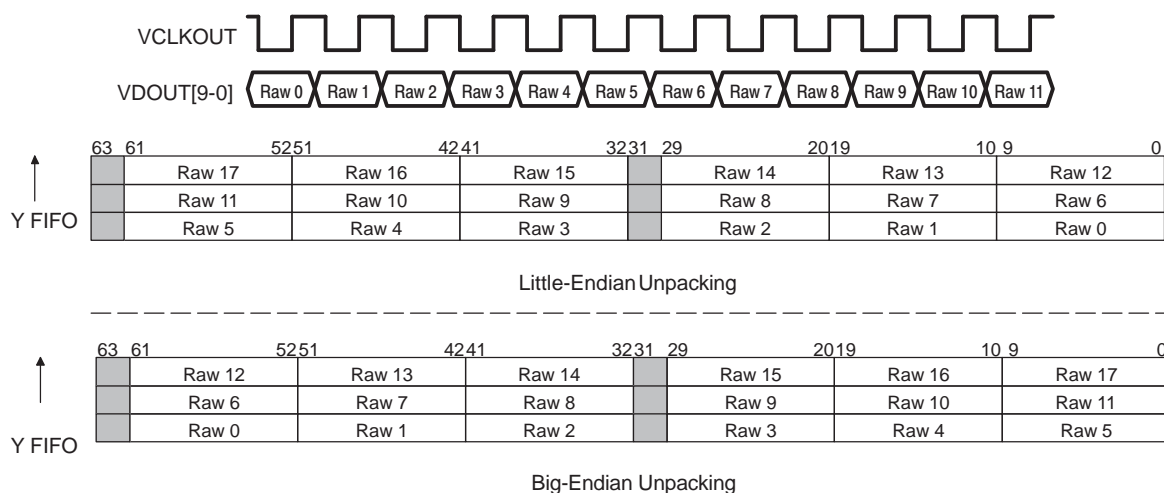
Figure 4-27. 10-Bit Raw Dense FIFO Unpacking
