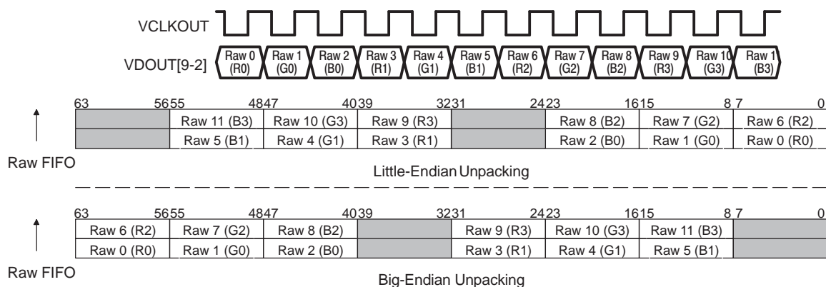
Figure 4-30. 8-Bit Raw \frac{3}{4} FIFO Unpacking
