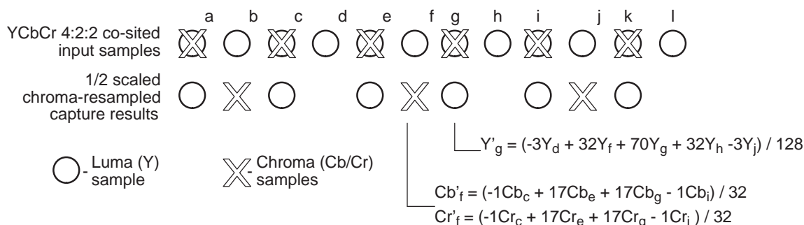
Figure 3-14. ½ Scaled Chrominance Re-sampled Filtering
