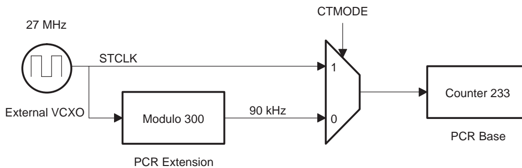
Figure 3-24. System Time Clock Counter Operation
