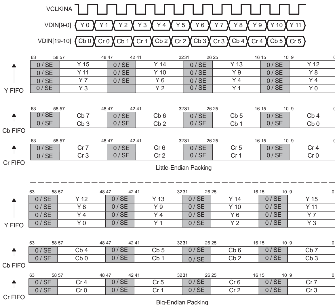
Figure 3-6. 10-Bit Y/C FIFO Packing
