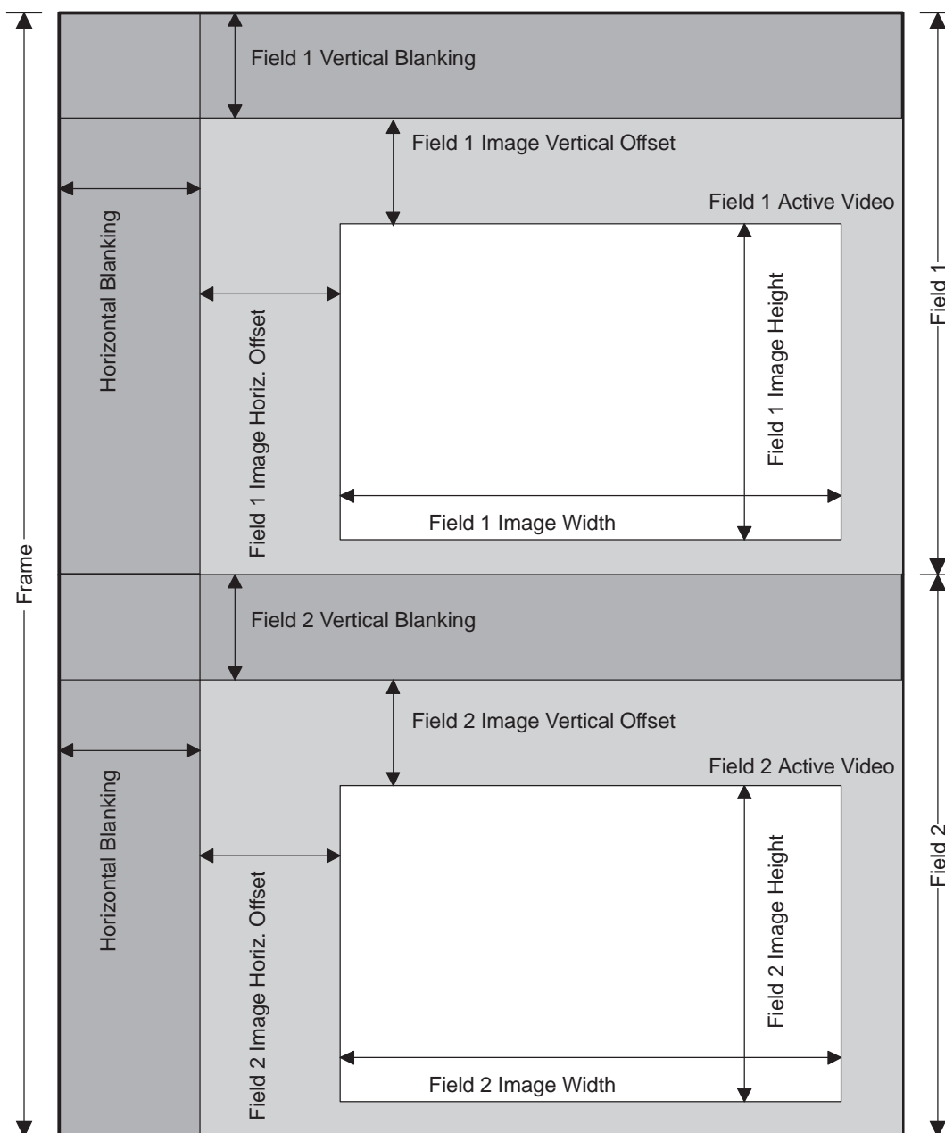
Figure 4-3. Interlaced Blanking Intervals and Video Areas
