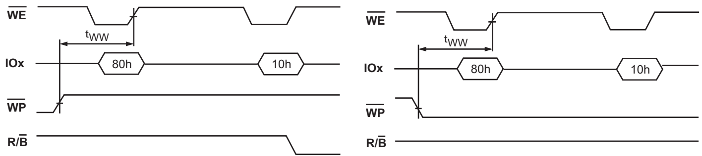
Figure 35: program Enabling / Disabling through WP# handling
