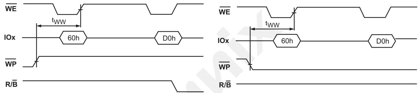
Figure 36: Erase Enabling / Disabling through WP# handling
