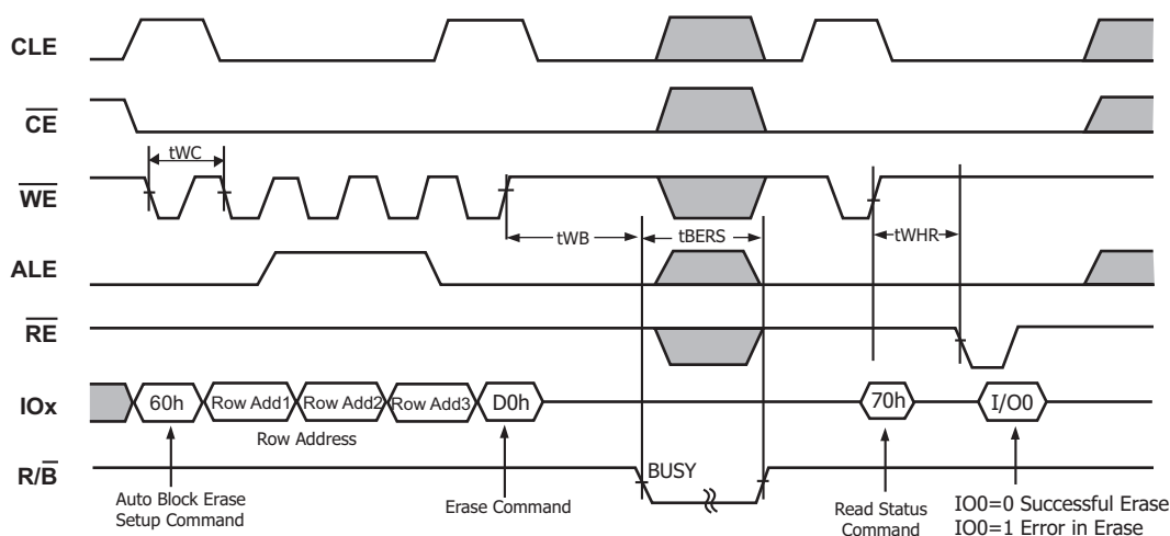
Figure 19: Block Erase Operation (Erase One Block)
