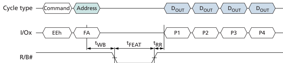
Figure 30: GET FEATURES (EEh) Operation
