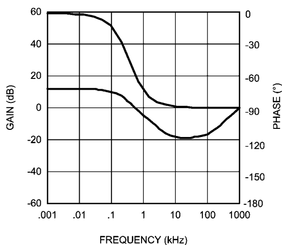
FIGURE 13. Modulator Gain and Phase
