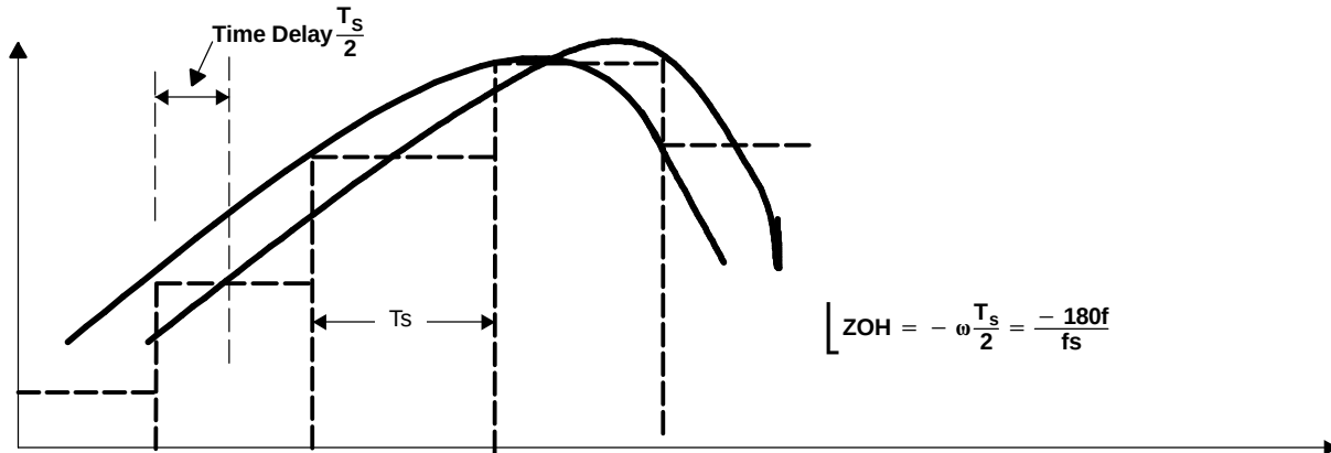
Figure 7. Sample and Hold Process in a Digital System
