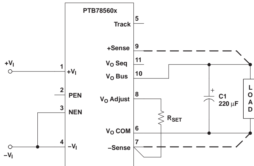
Figure 31. Stand-Alone Configuration
