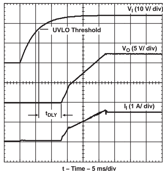
Figure 21. Soft-Start Waveform
