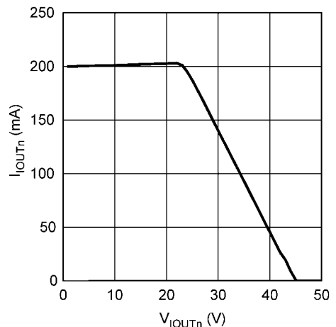
FIGURE 5. Over-power Protection
