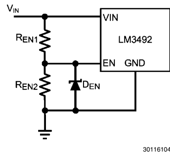
FIGURE 2. Input Voltage UVLO Implemented by Precision Enable
