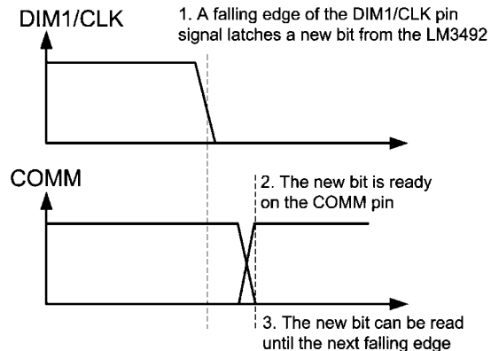
FIGURE 7. Read from the COMM Pin
