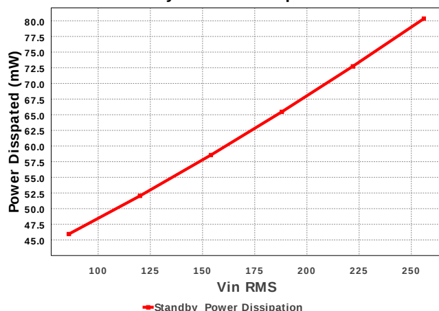
Standby Power Dissipation
