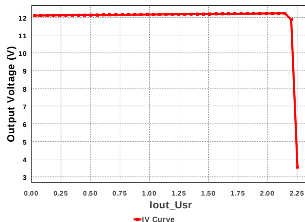
IV Curve
