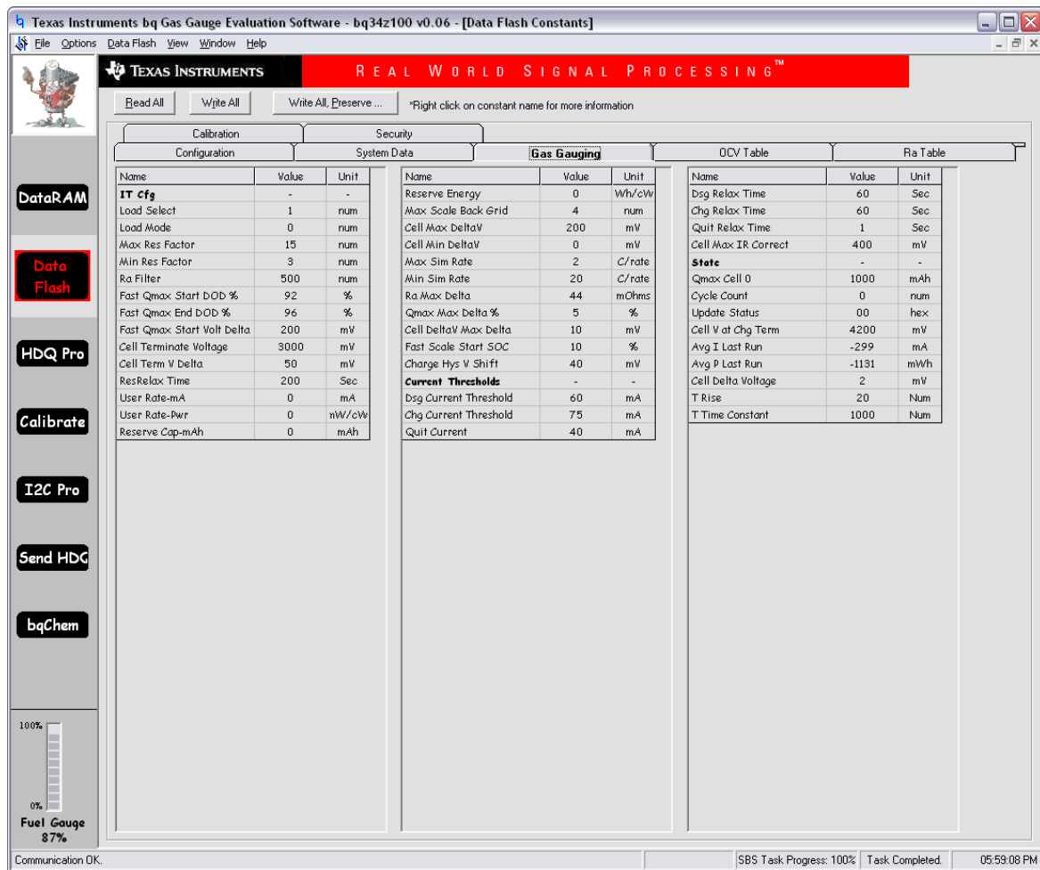
Figure 3. Gas Gauging Screen
