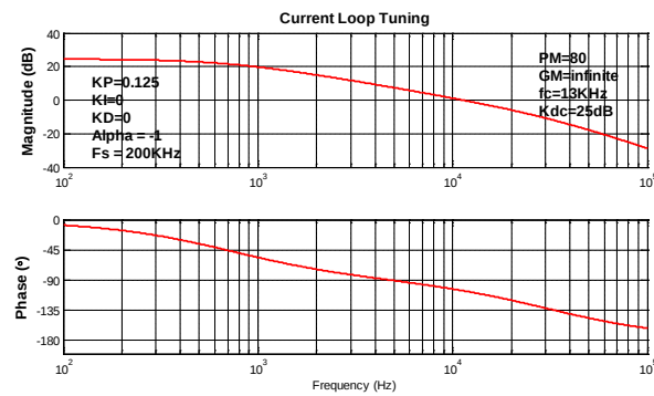
Figure 19: K_p Tuning – Bode Plot
