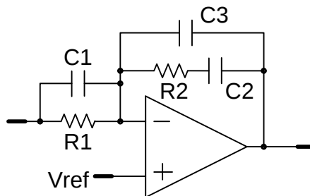
Figure 3: Traditional Analog Compensator
