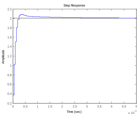
Figure 22: K_I Tuning – Step Response
