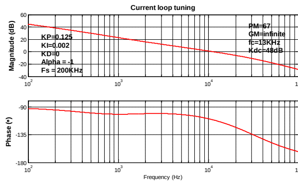
Figure 21: K_I Tuning – Bode Plot
