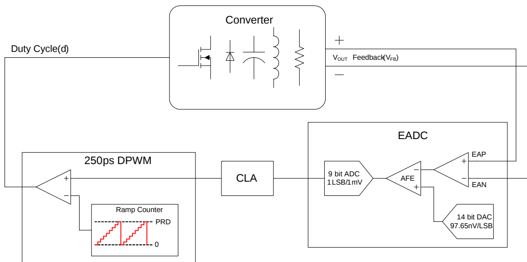
Figure 38: General UCD3138 Block Diagram
