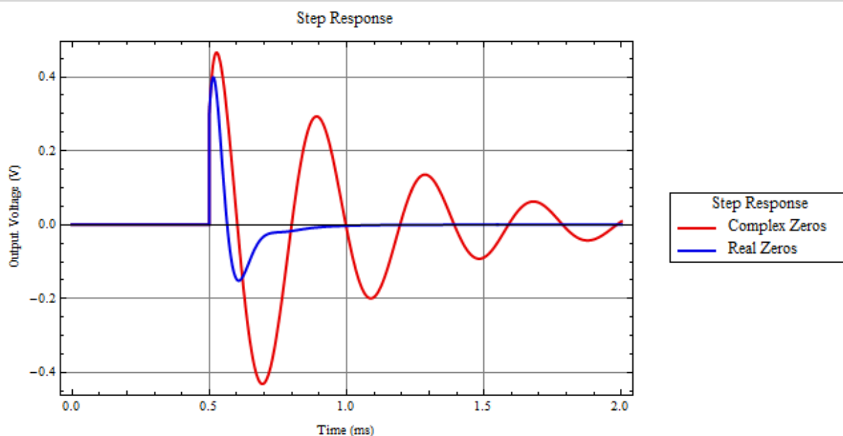
Figure 48: Load Step Response
