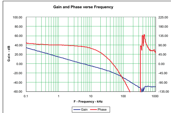
Figure 8. TPS40211EVM-352 Gain and Phase verse Frequency V_{IN} = 12\text{ V} , I_{OUT} = 0.70\text{ A} V_{OUT} = 24\text{ V} (8 white LEDs) V_{OUT} : Bandwidth: 5.7 kHz Phase Margin: 82^\circ
