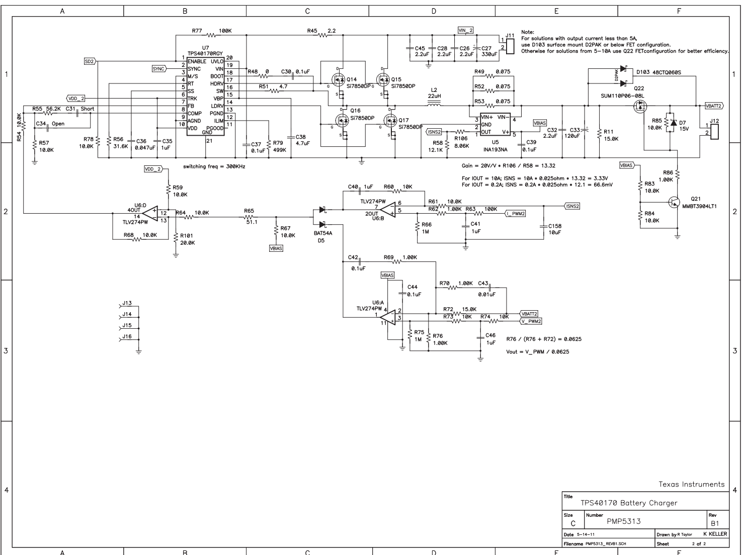
Figure 18. 60-V Input Power Stage Board Schematic (Page 2)
