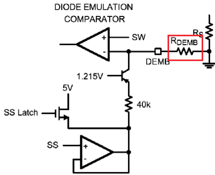
FIGURE 9. Diode Emulation Control
