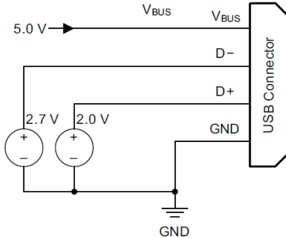
iPhone4 charger
