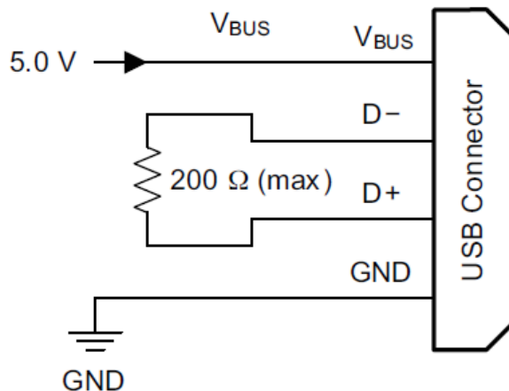
BC1.2 charger
