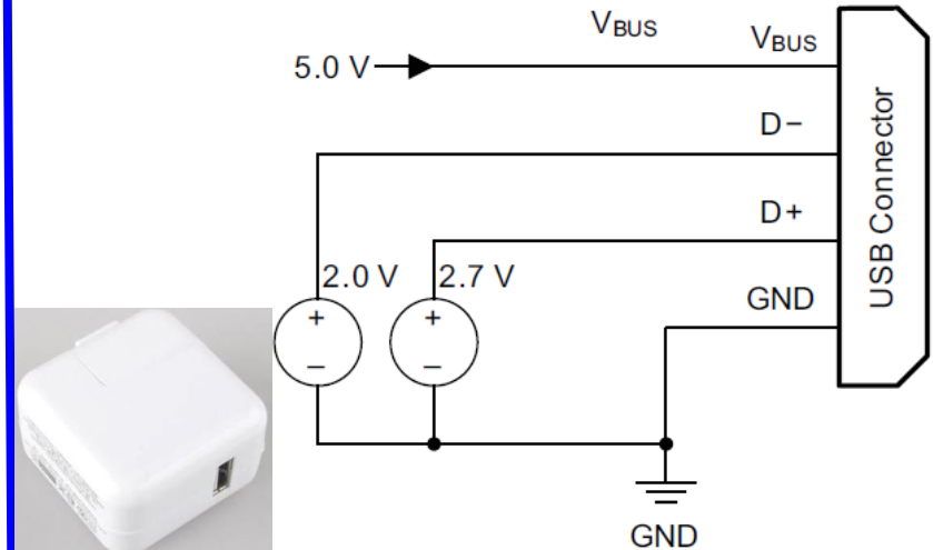
iPad charger
