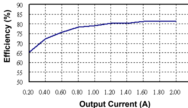
BUB12-48S1W Output Current vs. Efficiency
