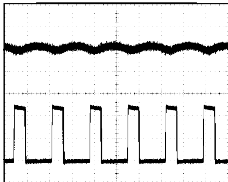
Switching Node and Output Voltage Waveforms
