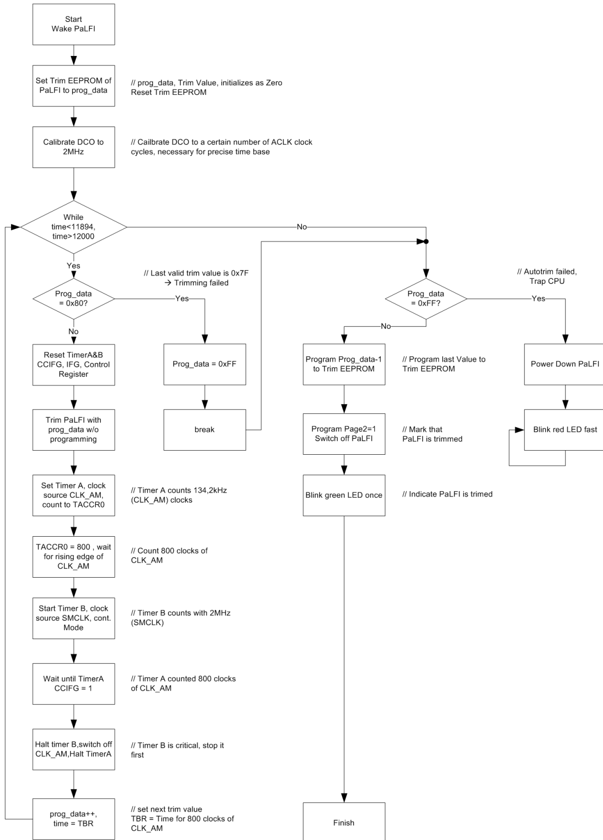
Figure 11. Autotrim Routine
