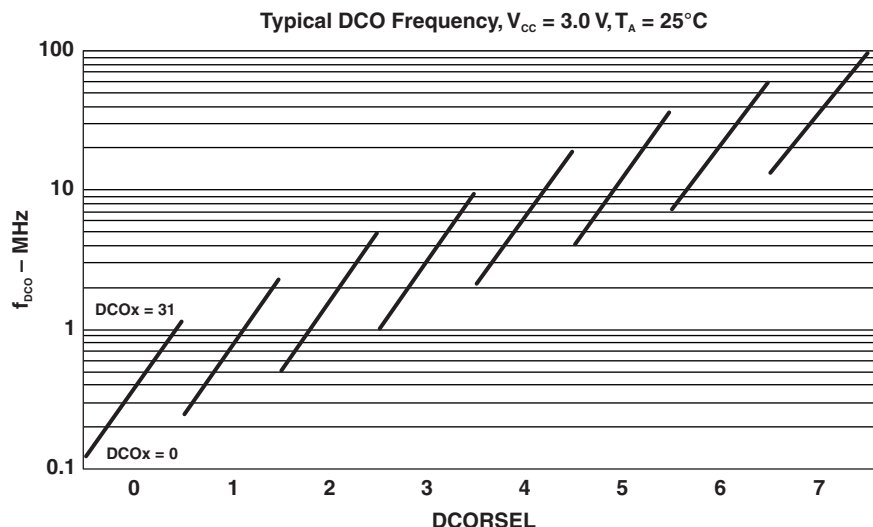
Figure 7. Typical DCO frequency
