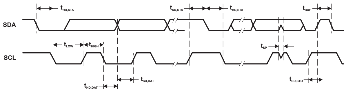
Figure 12. I2C Mode Timing
