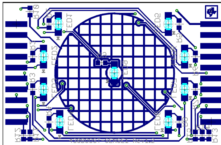
Figure 12. Capacitive Touch BoosterPack Layout, Bottom Layer and Silkscreen
