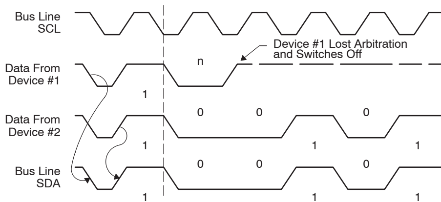
Figure 13–15. Arbitration Procedure Between Two Master Transmitters
