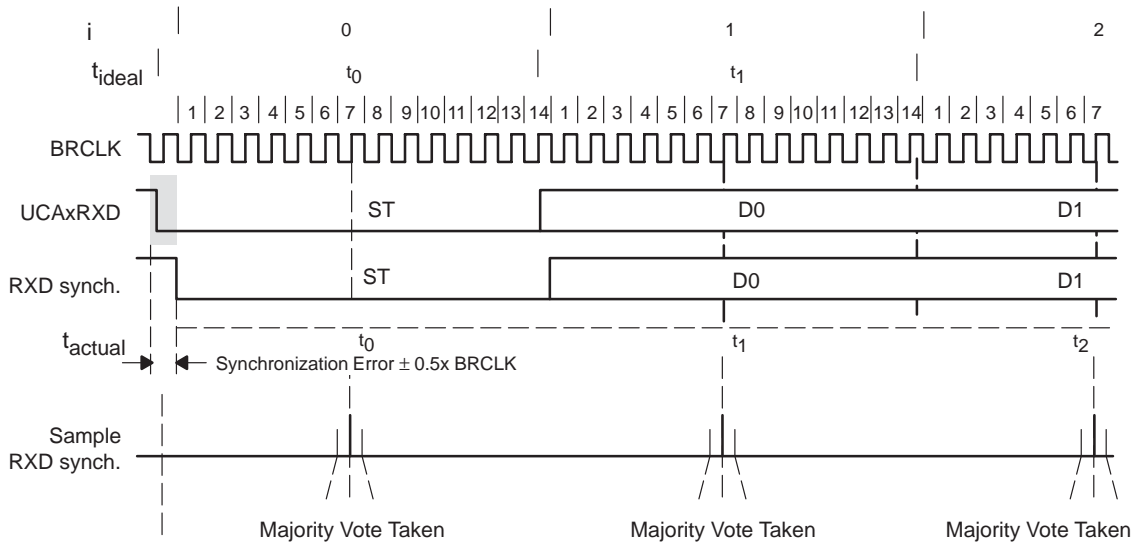
Figure 11–11. Receive Error
