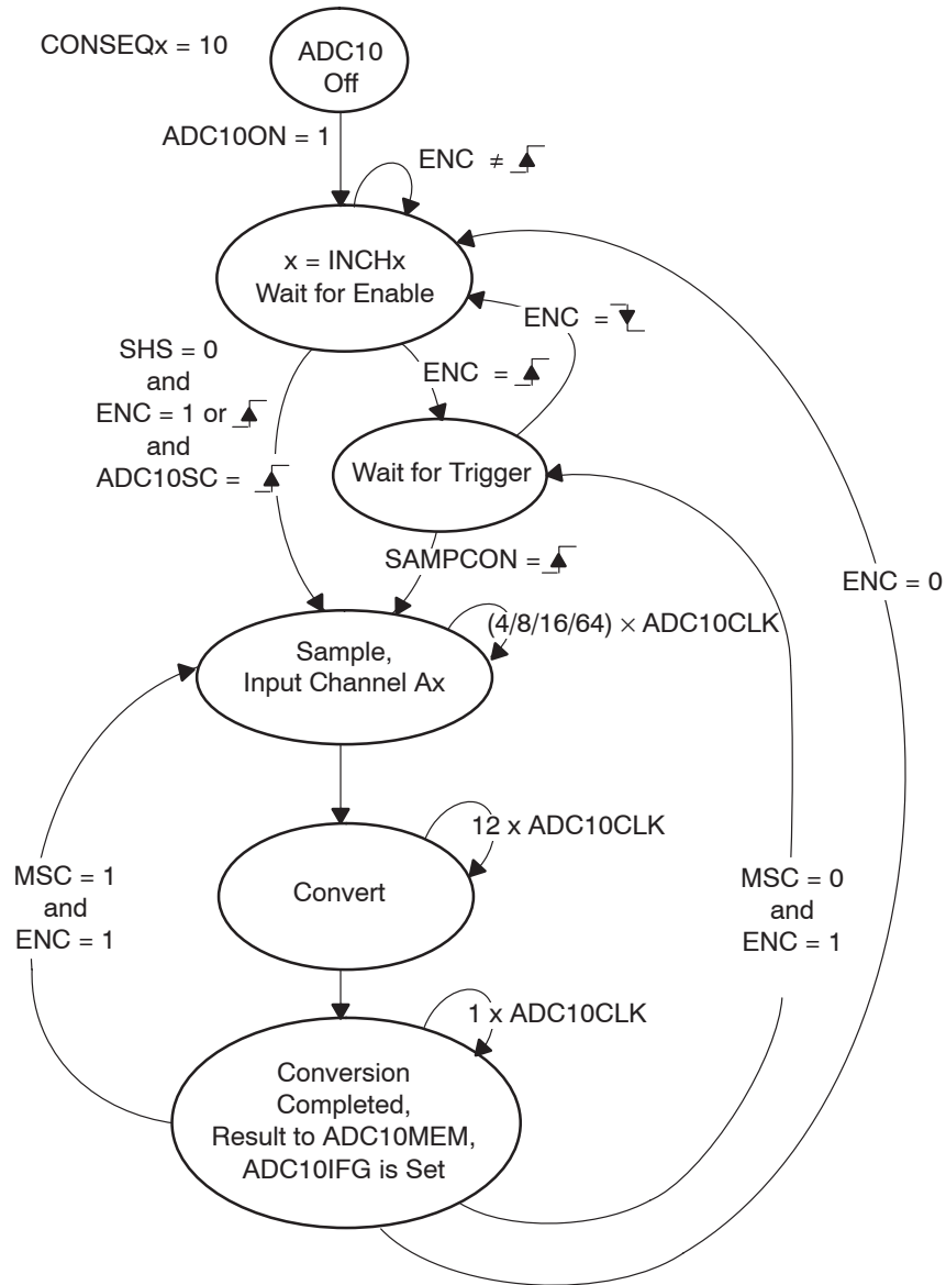
Figure 16–7. Repeat-Single-Channel Mode
