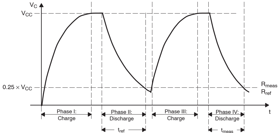
Figure 15–7. Timing for Temperature Measurement Systems
