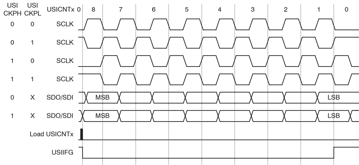
Figure 10–3. SPI Timing
