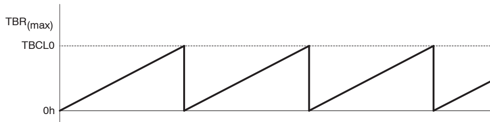
Figure 9–2. Up Mode
