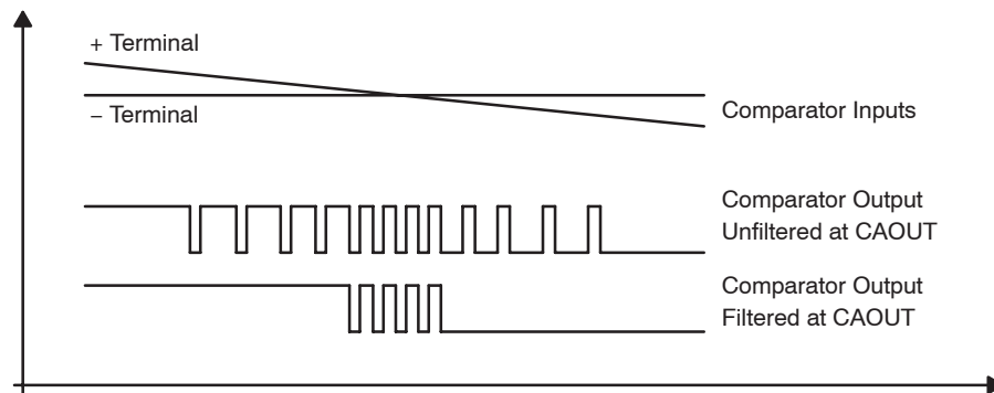
Figure 15–3. RC-Filter Response at the Output of the Comparator
