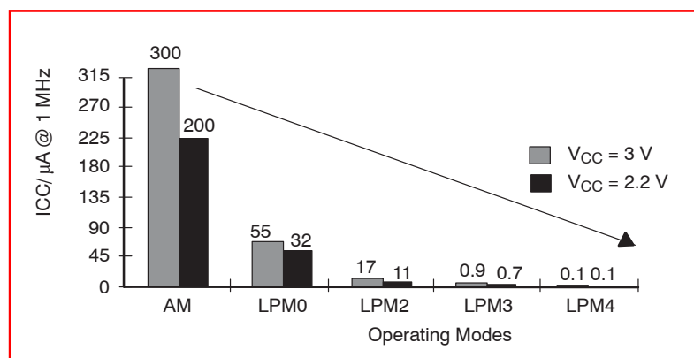
Figure 2–8. Typical Current Consumption of 21x1 Devices vs Operating Modes
