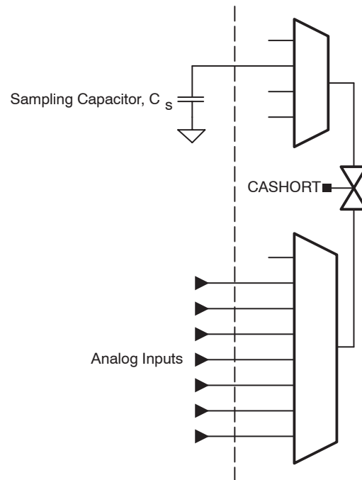
Figure 15-2. Comparator_A+ Sample-And-Hold
