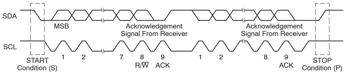
Figure 13–3. I 2 C Module Data Transfer
