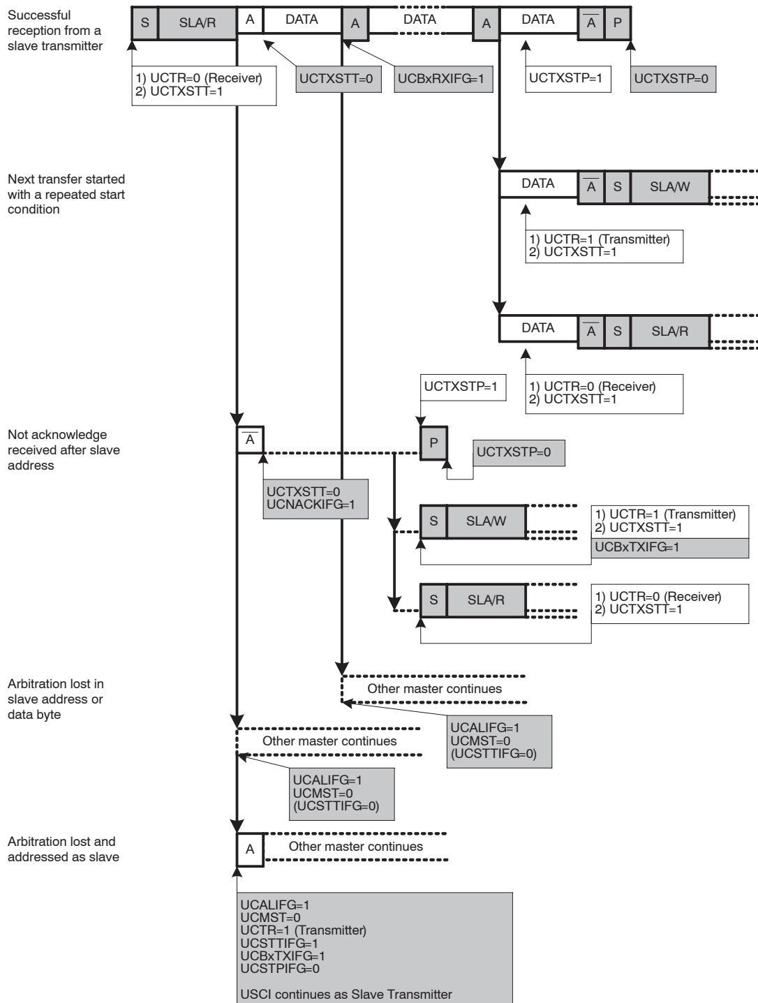
Figure 13–13. I 2 C Master Receiver Mode
