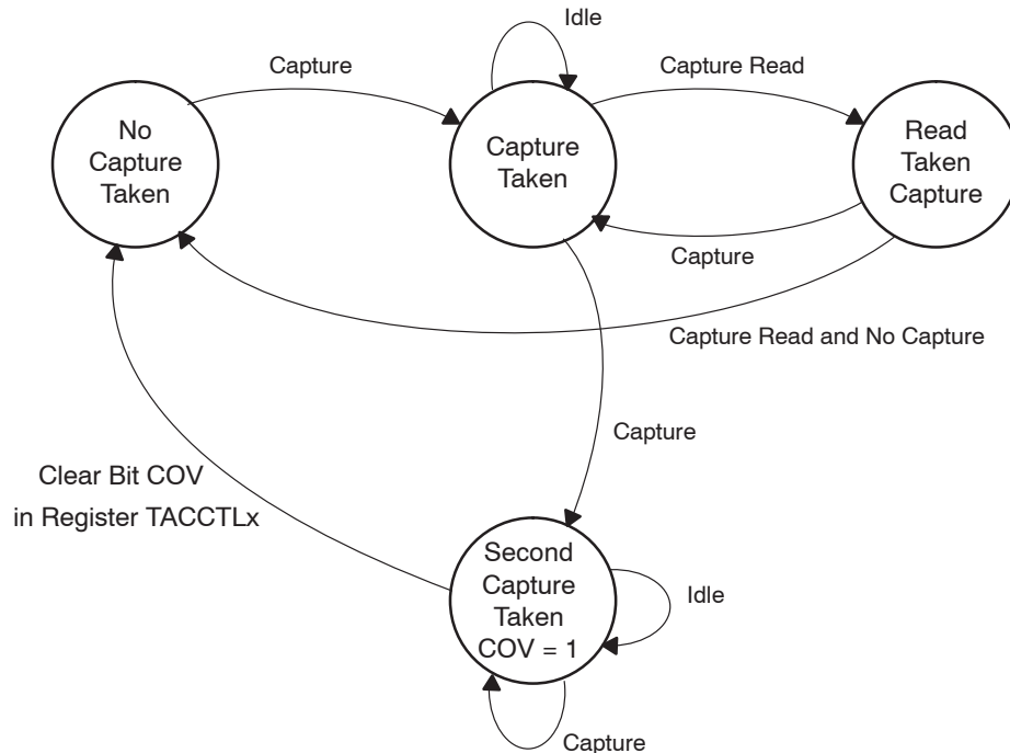
Figure 8–11. Capture Cycle
