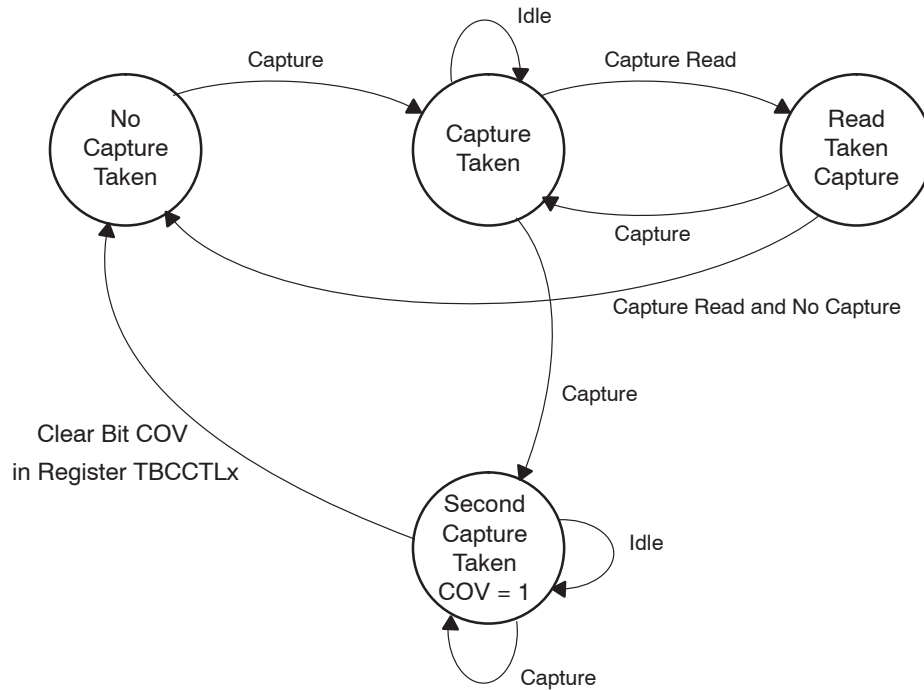
Figure 9–11. Capture Cycle
