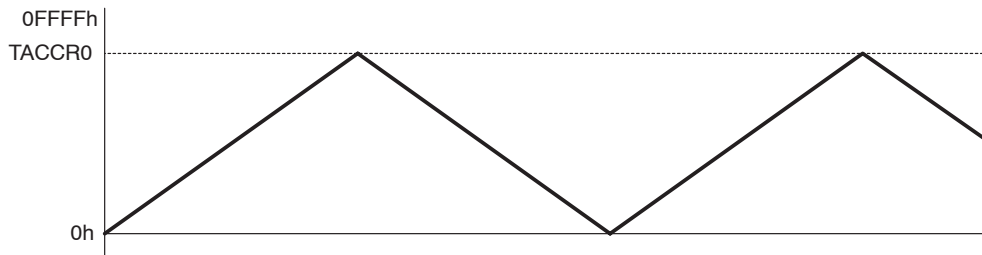
Figure 8–7. Up/Down Mode
