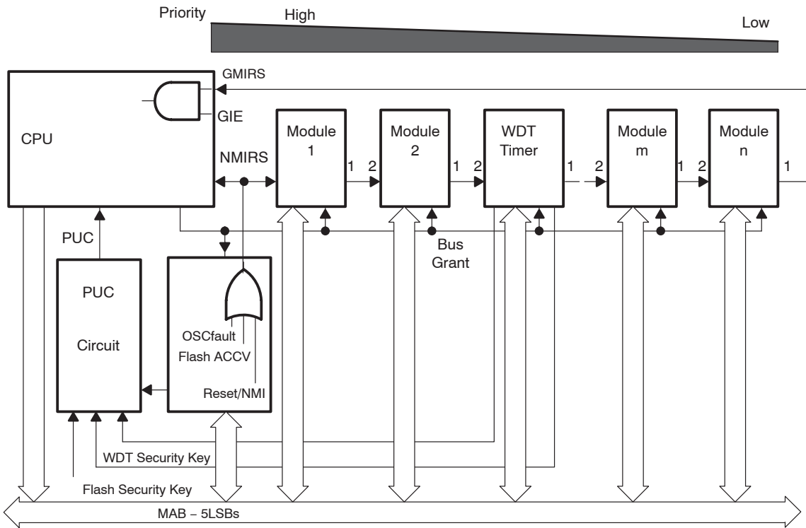
Figure 2–3. Interrupt Priority
