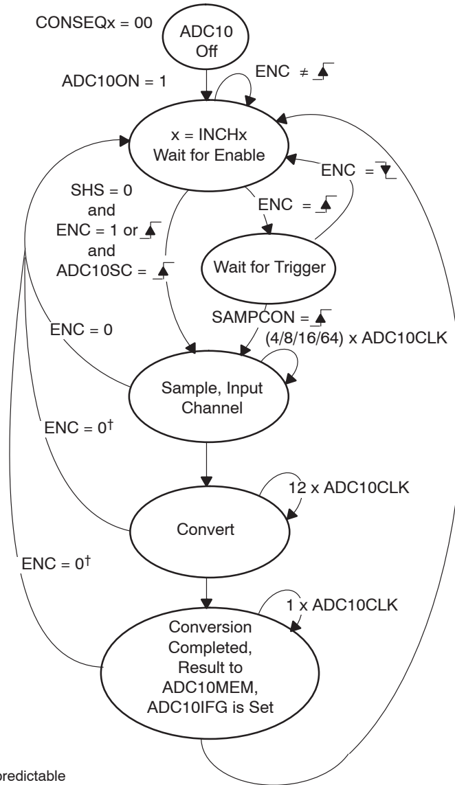
Figure 16-5. Single-Channel Single-Conversion Mode
