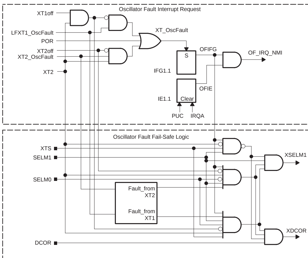
Figure 4–10. Oscillator-Fault-Interrupt
