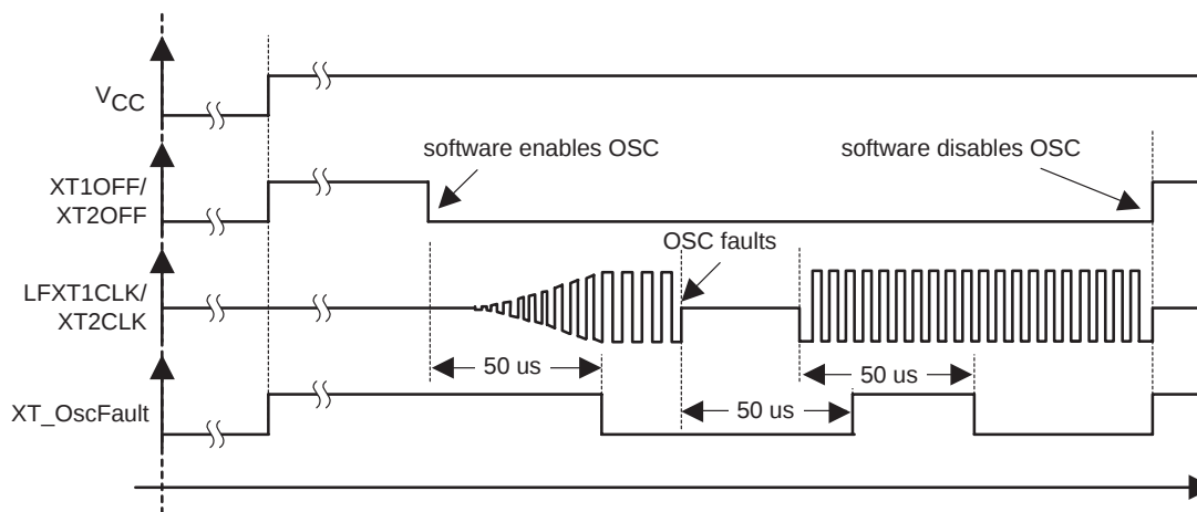
Figure 4–9. Oscillator-Fault Signal
