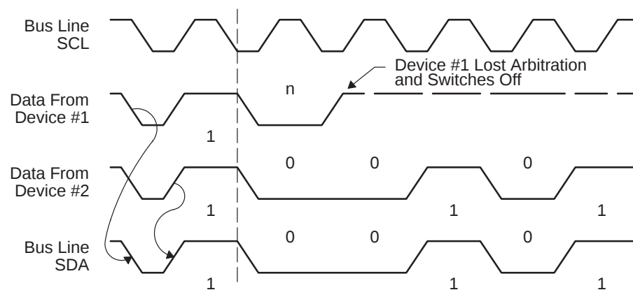
Figure 15–10. Arbitration Procedure Between Two Master Transmitters
