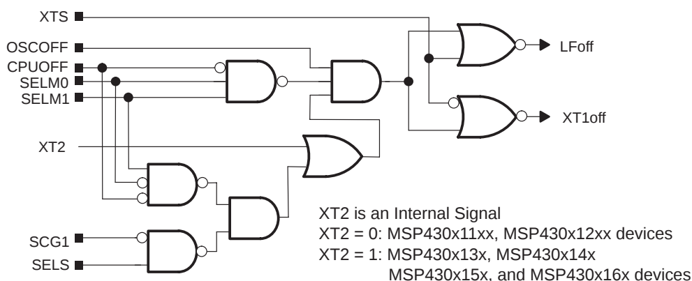
Figure 4-2. Off Signals for the LFXT1 Oscillator
