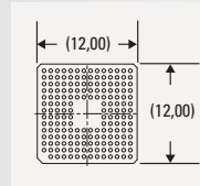
179-pin BGA
