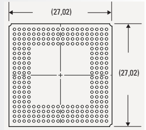
256-pin BGA
