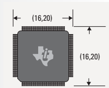
128-pin PQFP
