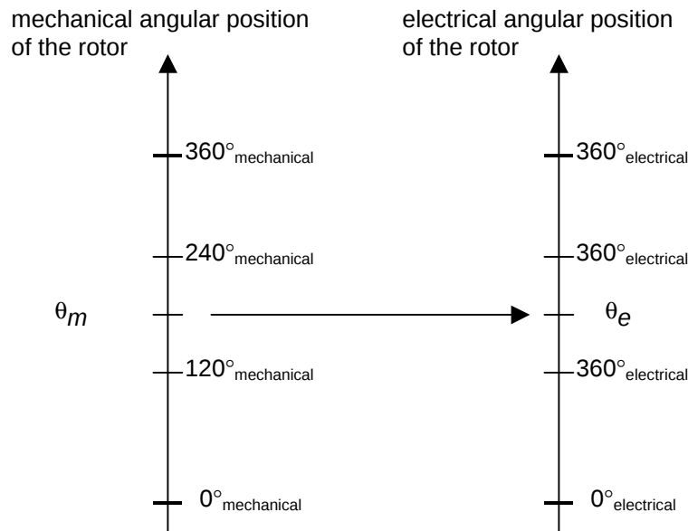
Figure 24. Electrical Position Scaling
