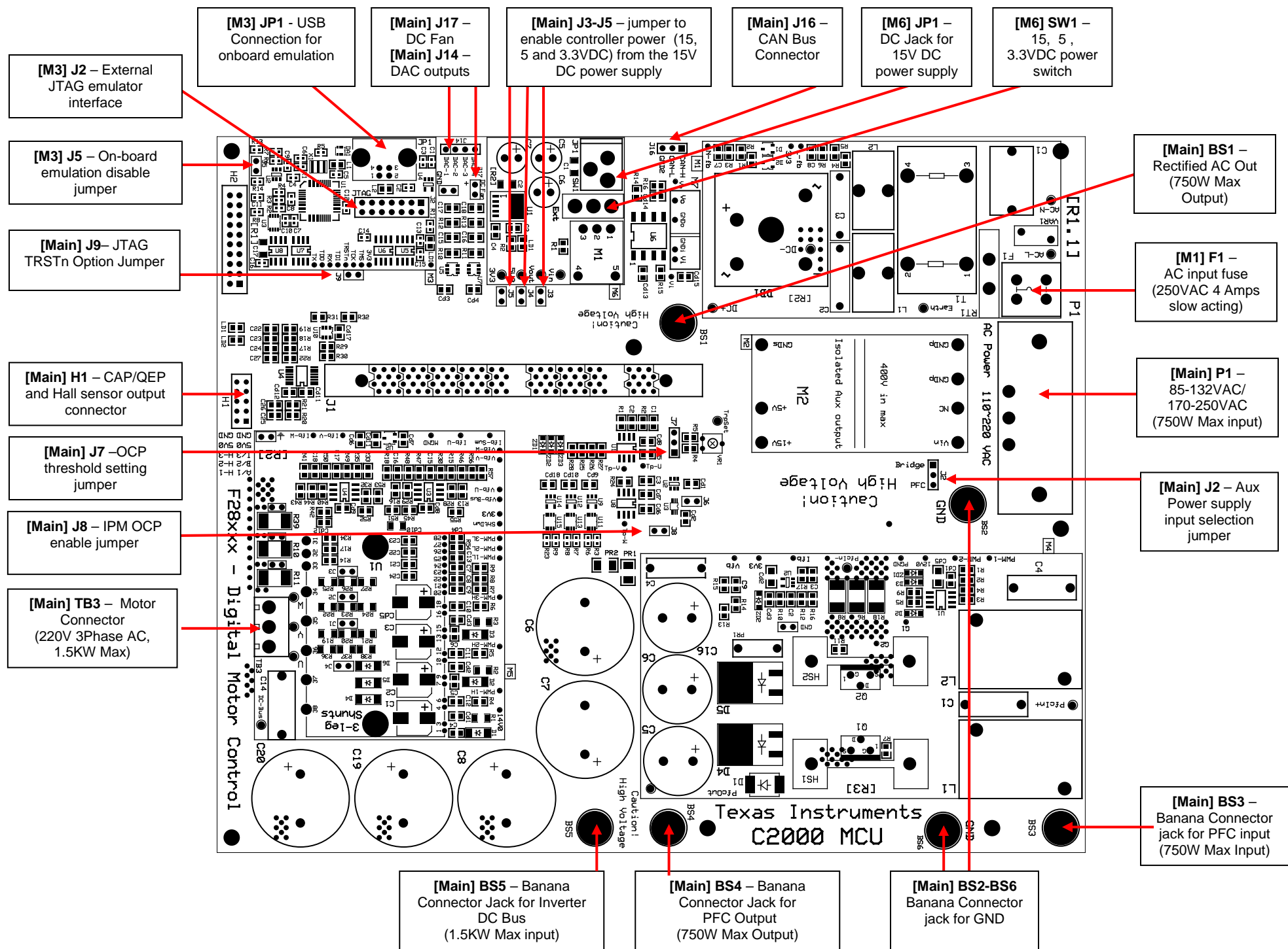
Fig5 HVMotorCtrl+PFC Kit Jumpers and Connectors Diagram
