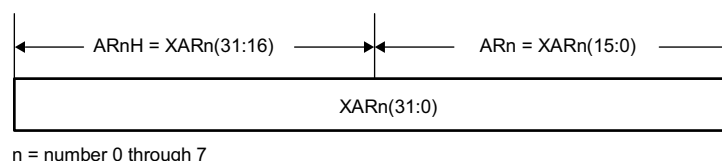
Figure 2-8. XAR0 - XAR7 Registers
