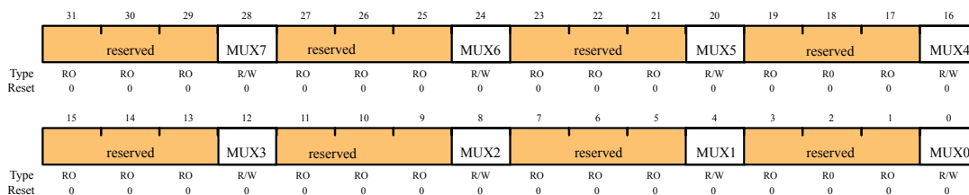
ADC 采样序列输入多路复用器选择0 (ADCSSMUX0) Offset 0x040
