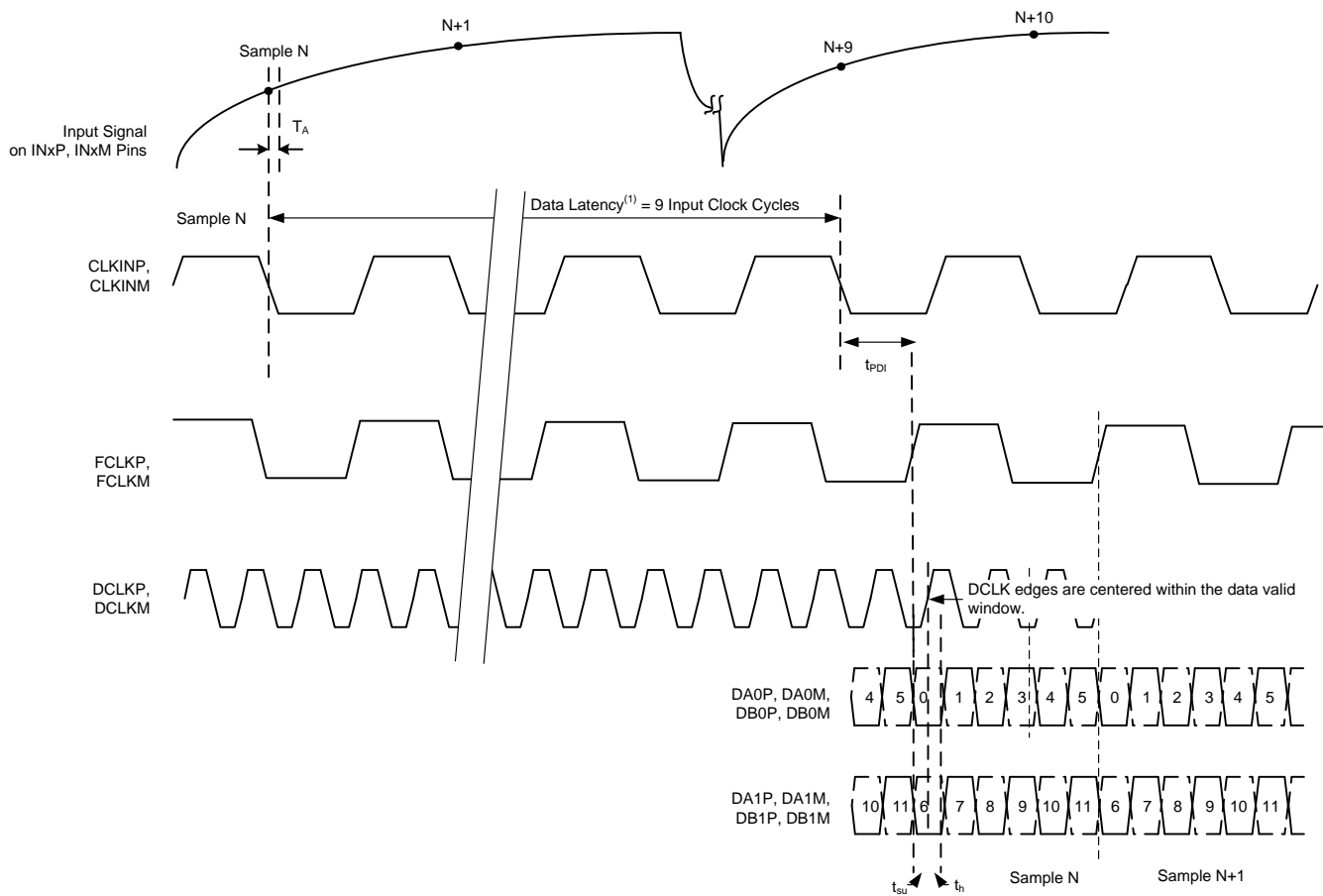
Figure 131. Latency Diagram
