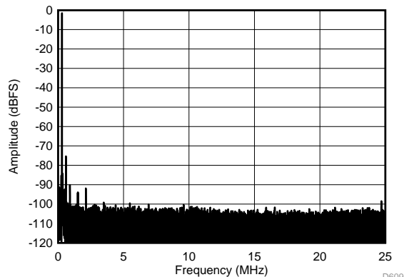
D609 SFDR = 68.2 dBc, SNR = 67.4 dBFS, SINAD = 67.3 dBFS, THD = -86.4 dBc, HD2 = -68.2 dBc, HD3 = -87.3 dBc
