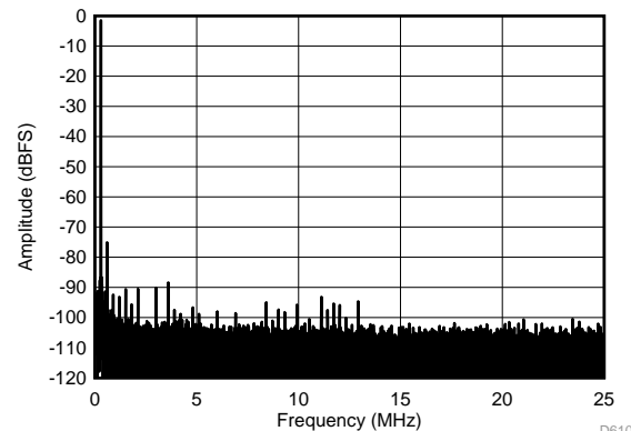
D610 SFDR = 68.1 dBc, SNR = 67.7 dBFS, SINAD = 67.6 dBFS, THD = -86.6 dBc, HD2 = 68.1 dBc, HD3 = -87.3 dBc
