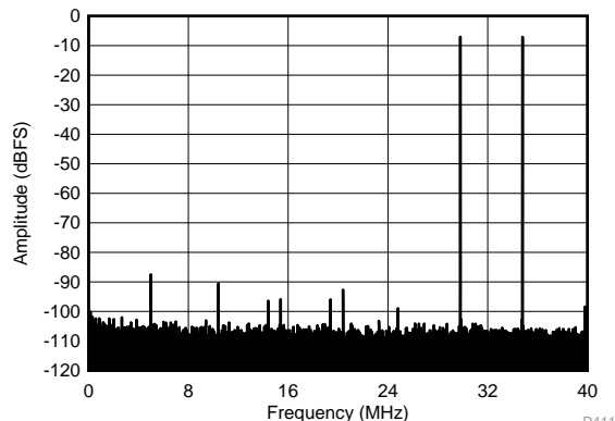
f_{IN1} = 46 \text{ MHz} , f_{IN2} = 50 \text{ MHz} , IMD3 = 87.5 dBFS, each tone at -7 dBFS
