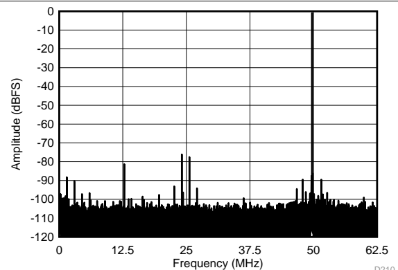
SFDR = 75.2 dBc, SNR = 68 dBFS, SINAD = 67.0 dBFS, THD = 72.5 dBc, HD2 = -76.5 dBc, HD3 = -75.2 dBc
