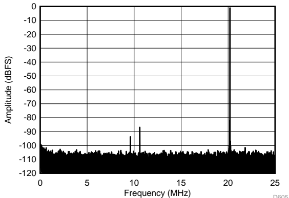
SFDR = 85.9 dBc, SFDR = 99.1 dBc (non 23), SNR = 70.4 dBFS, SINAD = 70.2 dBFS, THD = 84.8 dBc, HD2 = -92.7 dBc, HD3 = -85.9 dBc
