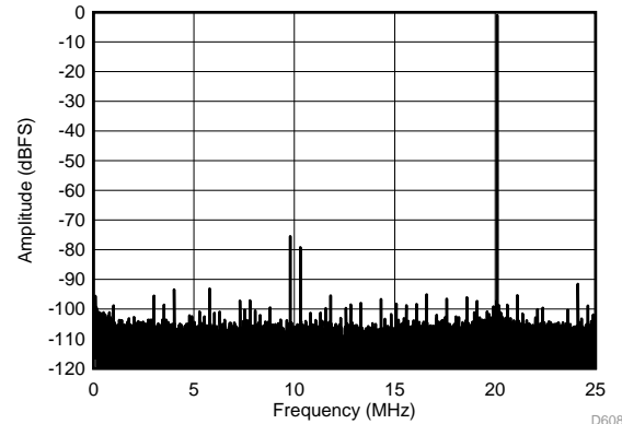
D608 SFDR = 74.5 dBc, SFDR = 91.1 dBc (non 23), SNR = 69.4 dBFS, SINAD = 68.1 dBFS, THD = 72.9 dBc, HD2 = -74.5 dBc, HD3 = -78.2 dBc
