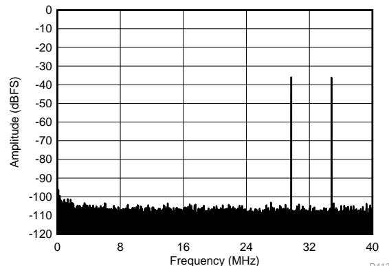
f_{IN1} = 46 \text{ MHz} , f_{IN2} = 50 \text{ MHz} , IMD3 = 95.7 dBFS, each tone at -36 dBFS
