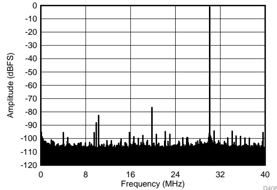
SFDR = 75.6 dBc, SNR = 69.7 dBFS, SINAD = 68.6 dBFS, THD = 74.5 dBc, HD2 = -75.6 dBc, HD3 = -81.6 dBc
