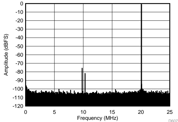
D607 SFDR = 74.7 dBc, SFDR = 95.2 dBc (non 23), SNR = 69.2 dBFS, SINAD = 68.1 dBFS, THD = 73.7 dBc, HD2 = -74.7 dBc, HD3 = -80.9 dBc
