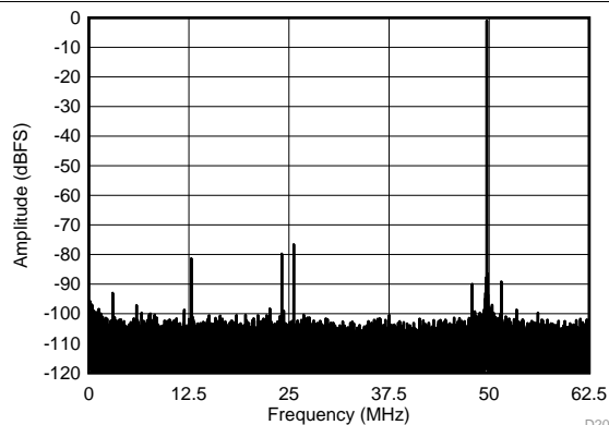
SFDR = 75.5 dBc, SNR = 67.4 dBFS, SINAD = 66.7 dBFS, THD = 73.8 dBc, HD2 = -75.5 dBc, HD3 = -78.7 dBc
