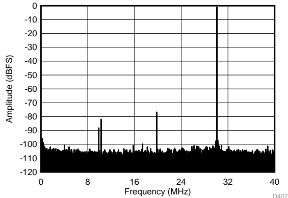
SFDR = 75.8 dBc, SNR = 69.4 dBFS, SINAD = 68.5 dBFS, THD = 74.6 dBc, HD2 = -75.8 dBc, HD3 = -80.9 dBc
