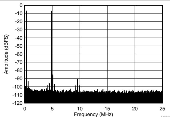
D611 f_{IN1} = 46 \text{ MHz} , f_{IN2} = 50 \text{ MHz} , IMD3 = 85.4 dBFS, each tone at -7 dBFS
