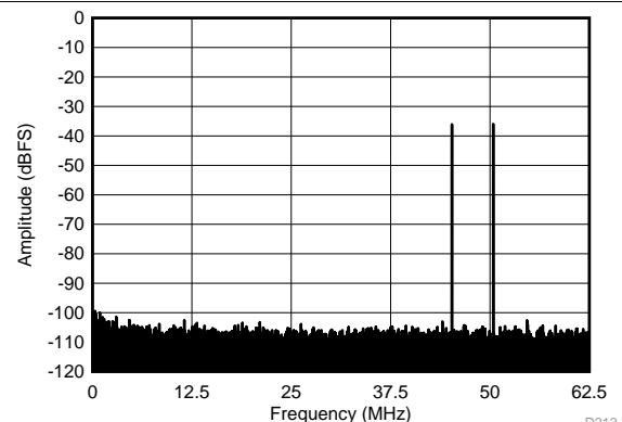
f_{IN1} = 46\text{ MHz} , f_{IN2} = 50\text{ MHz} , IMD3 = -96.7 dBFS, each tone at -36 dBFS
