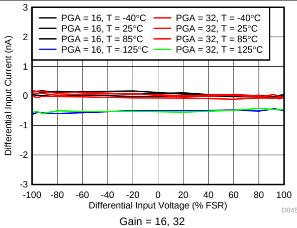
Figure 30. Differential Input Current vs Differential Input Voltage
