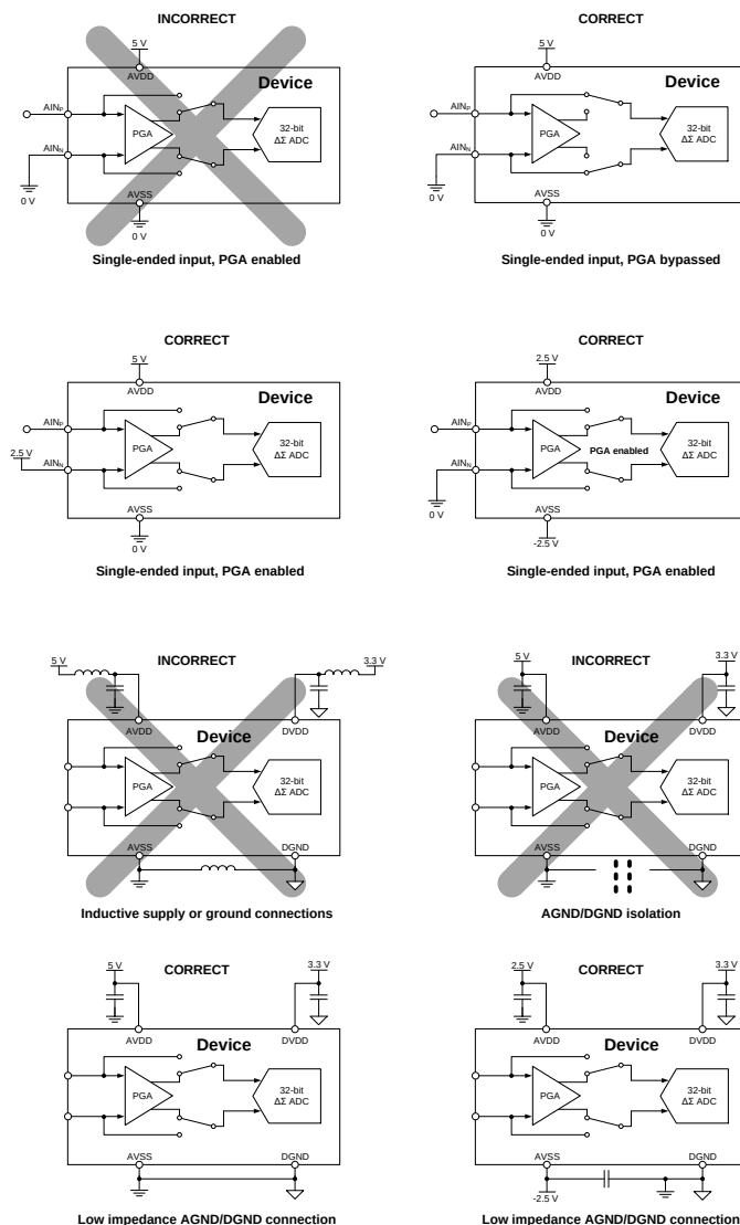
Figure 140. Do's and Don'ts Diagrams
