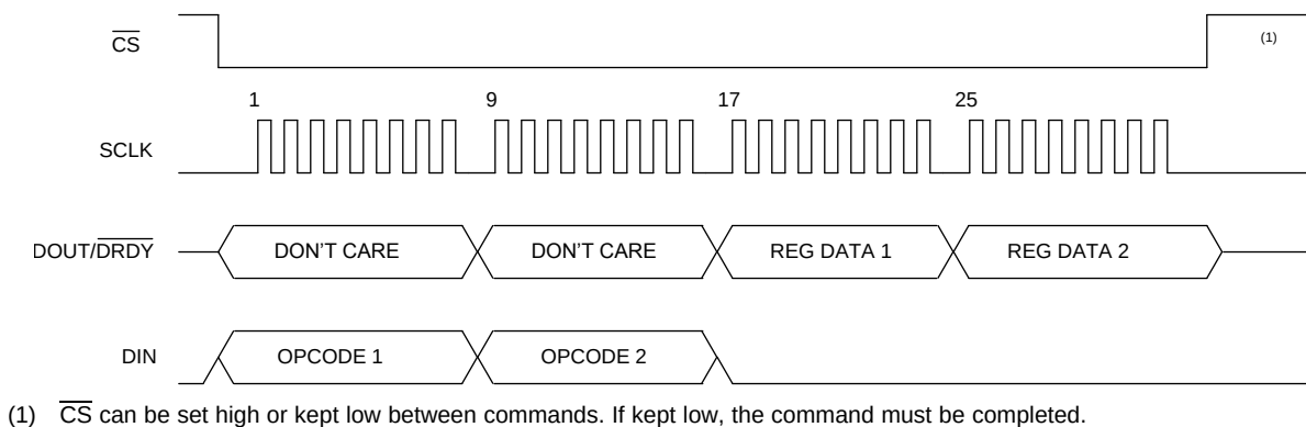
Figure 103. Read Register Sequence
