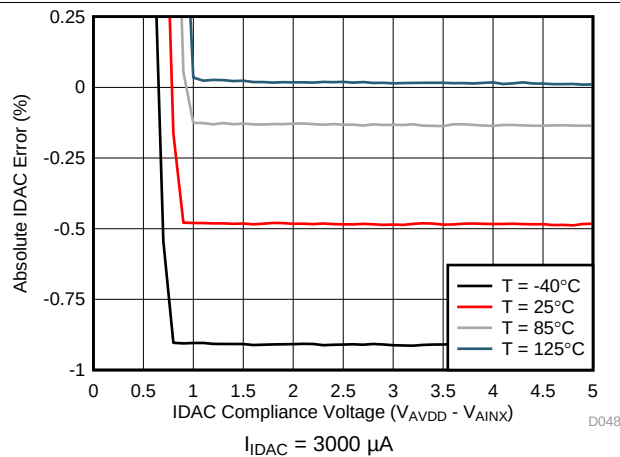
Figure 36. IDAC Error vs Compliance Voltage
