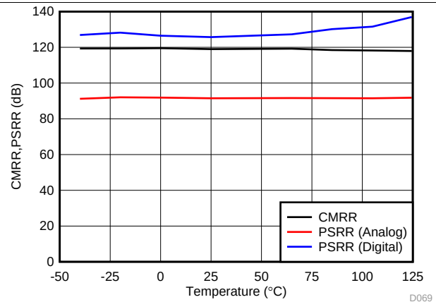
Figure 35. CMRR, PSRR vs Temperature
