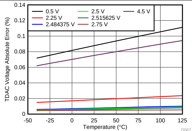
Figure 47. TDAC Error vs Temperature
