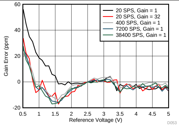
Figure 11. Gain Error vs Reference Voltage
