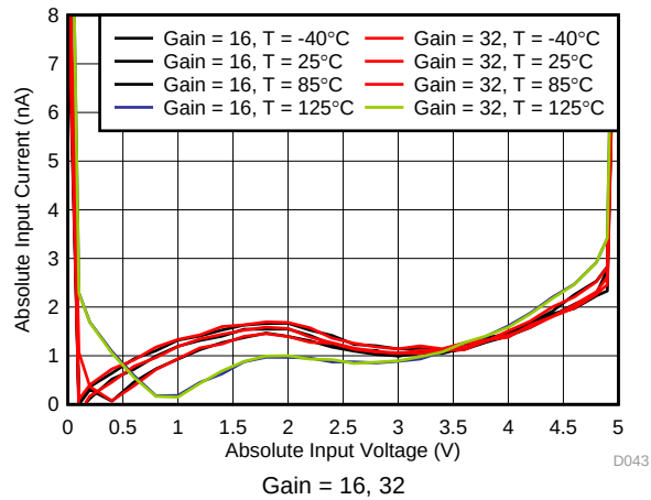
Figure 28. Absolute Input Current vs Absolute Input Voltage
