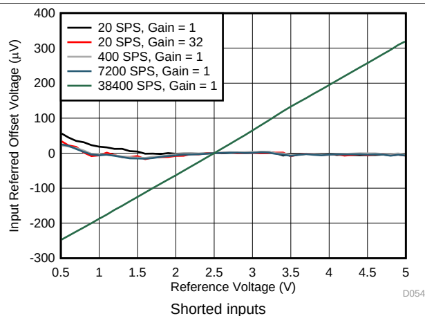
Figure 8. Offset Voltage vs Reference Voltage
