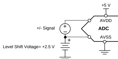
Figure 126. Single-Ended Input with Offset
