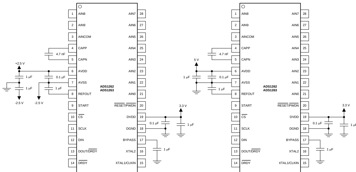
Figure 142. Power-Supply Decoupling
