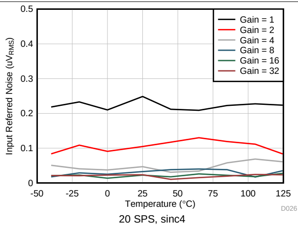
Figure 12. Noise vs Temperature
