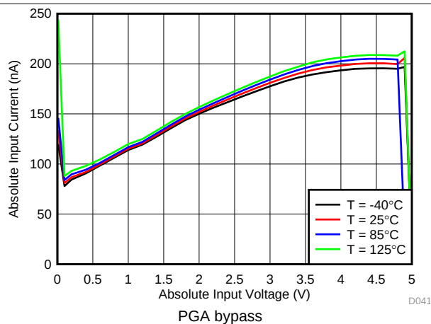
Figure 26. Absolute Input Current vs Absolute Input Voltage
