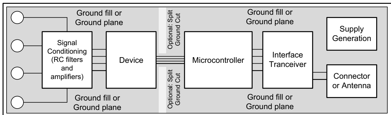
Figure 144. System Component Placement
