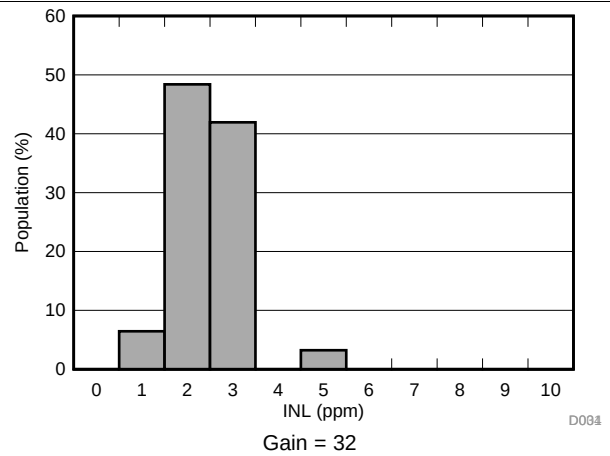
Figure 23. INL Distribution
