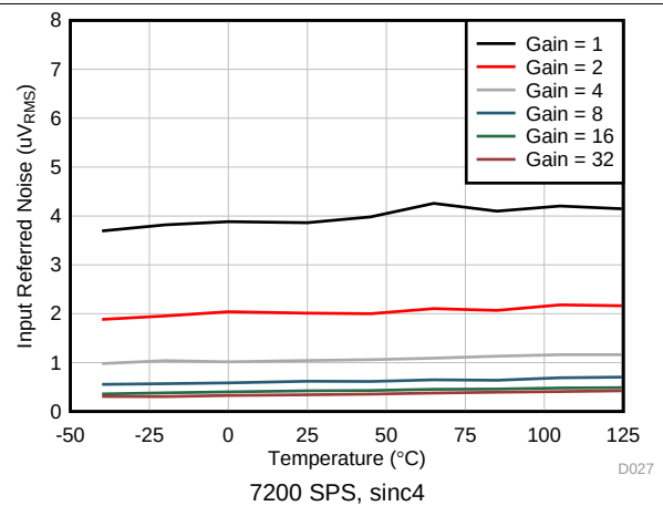
Figure 13. Noise vs Temperature
