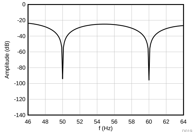
Figure 80. ADC2 10 SPS Frequency Response 50/60 Hz Detail
