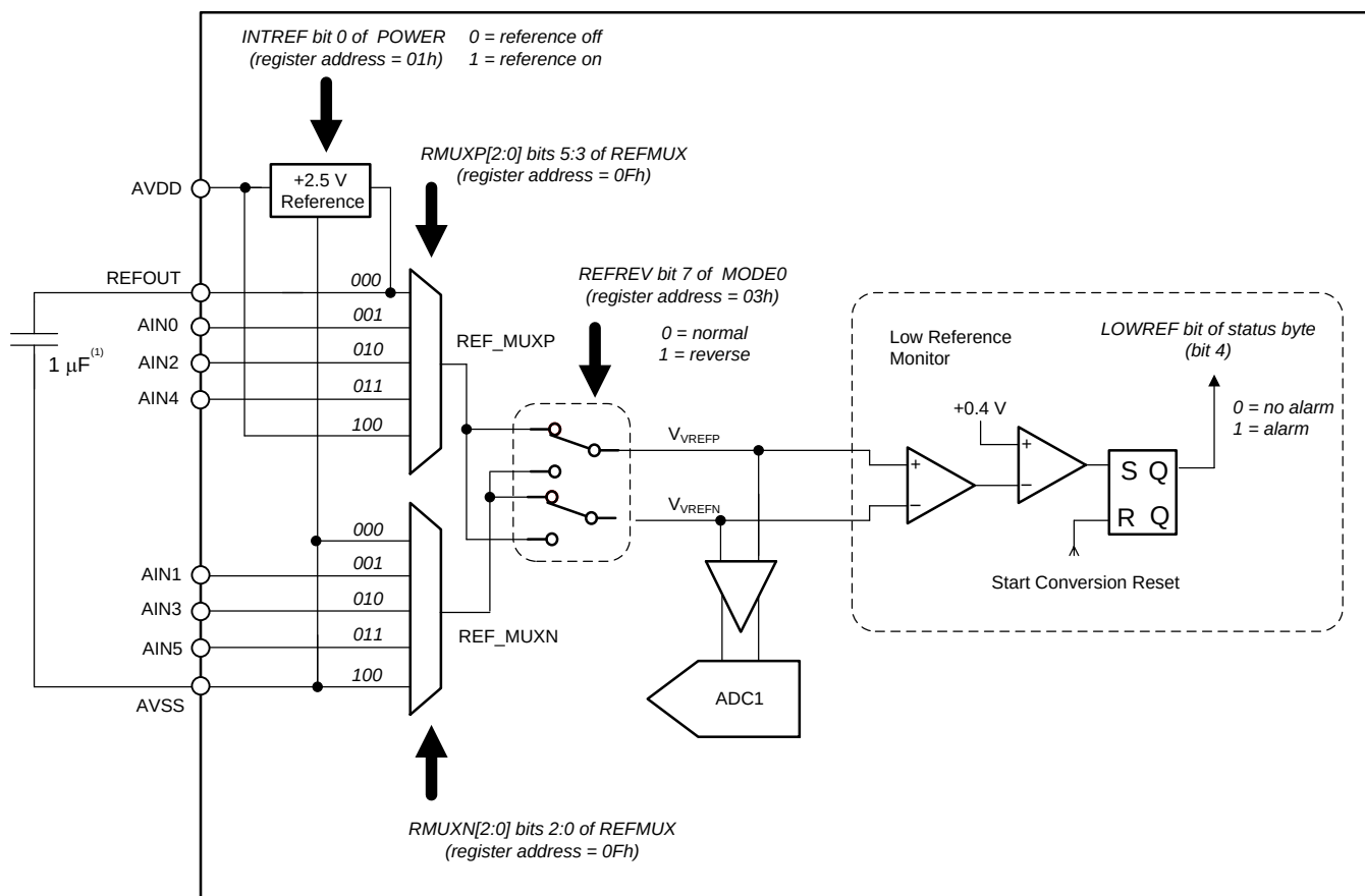
Figure 59. ADC1 Reference Multiplexer Block Diagram
