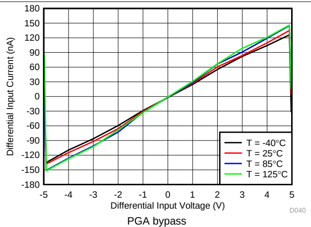
Figure 25. Differential Input Current vs Differential Input Voltage
