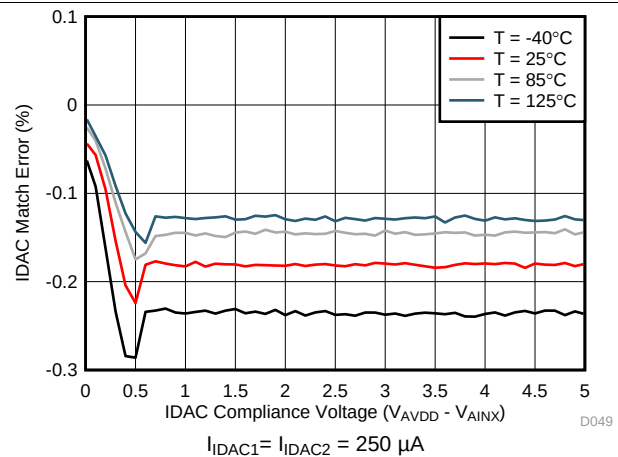
Figure 37. IDAC Error vs Compliance Voltage
