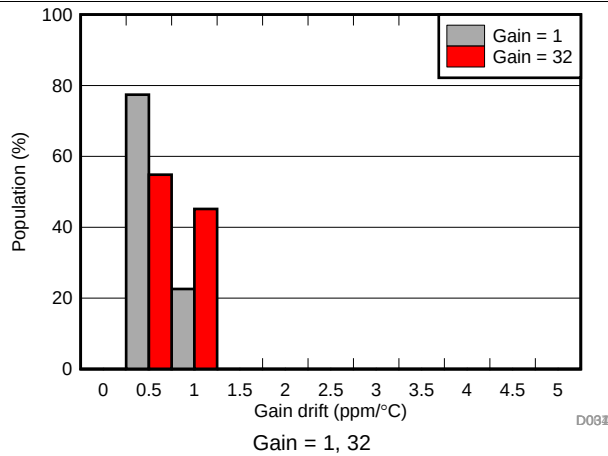
Figure 10. Gain vs Temperature Distribution
