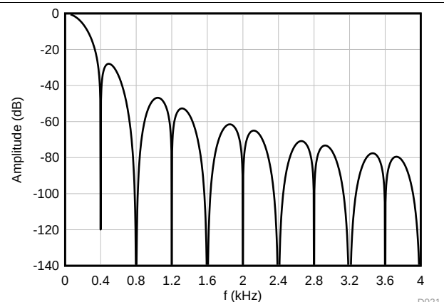
Figure 82. ADC2 400 SPS Frequency Response
