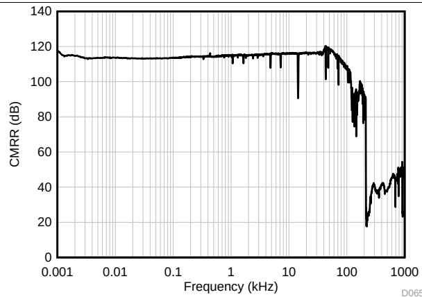
Figure 34. CMRR vs Frequency
