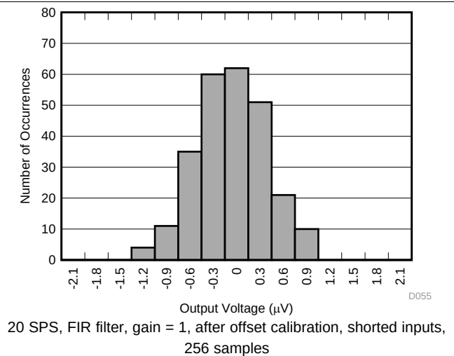
Figure 15. Output Reading Distribution
