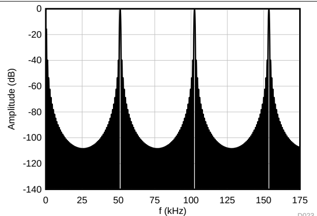
Figure 84. ADC2 Frequency Response to 175 kHz
