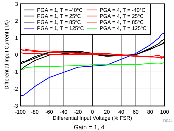
Figure 29. Differential Input Current vs Differential Input Voltage
