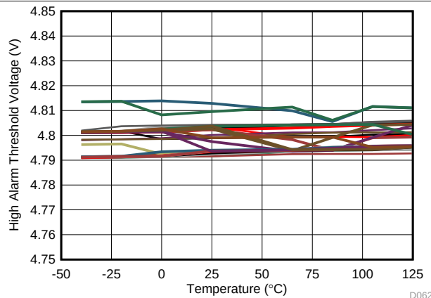
Figure 46. PGA Absolute High Alarm Threshold vs Temperature
